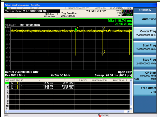
802.11ax-HE20_242 Tone_RU122
