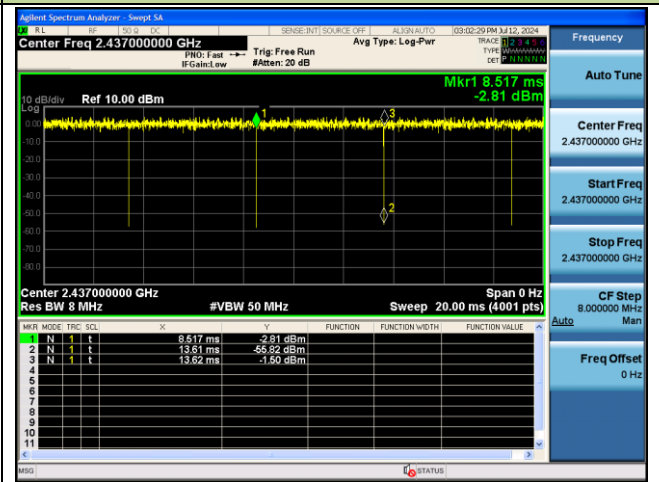
802.11ax-HE20_242 Tone_RU122
