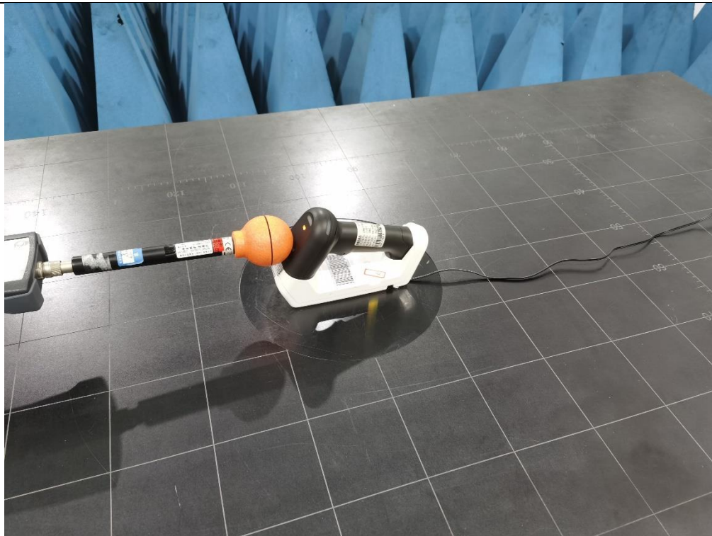
Description: RF Exposure Setup (Above 100kHz) - ISED
