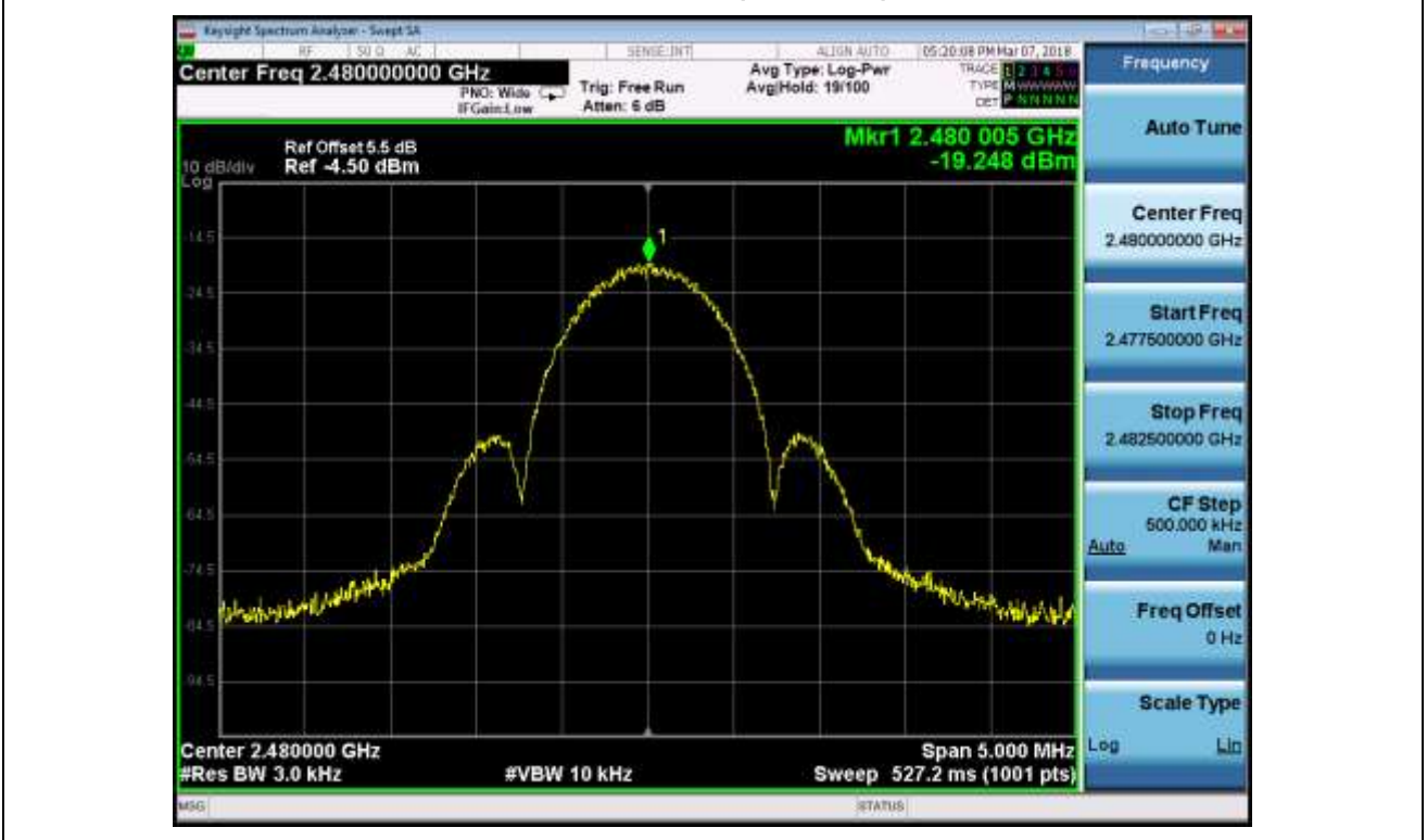
Mode 1 CH39(2480MHz)
