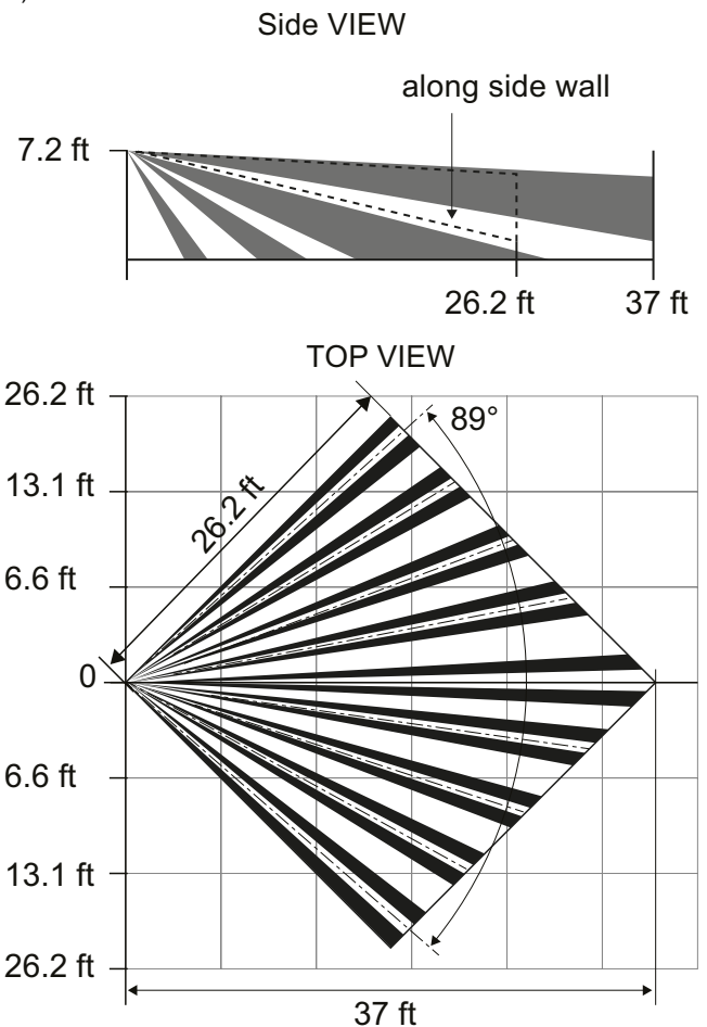
Figure 3 EN1263 detection coverage area
