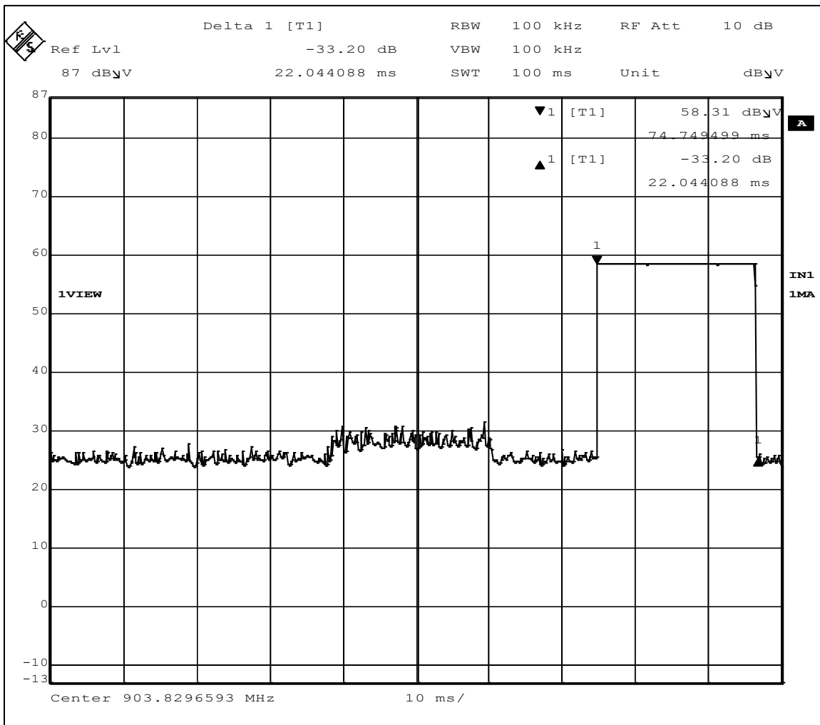
Figure 2 – Duty Cycle
