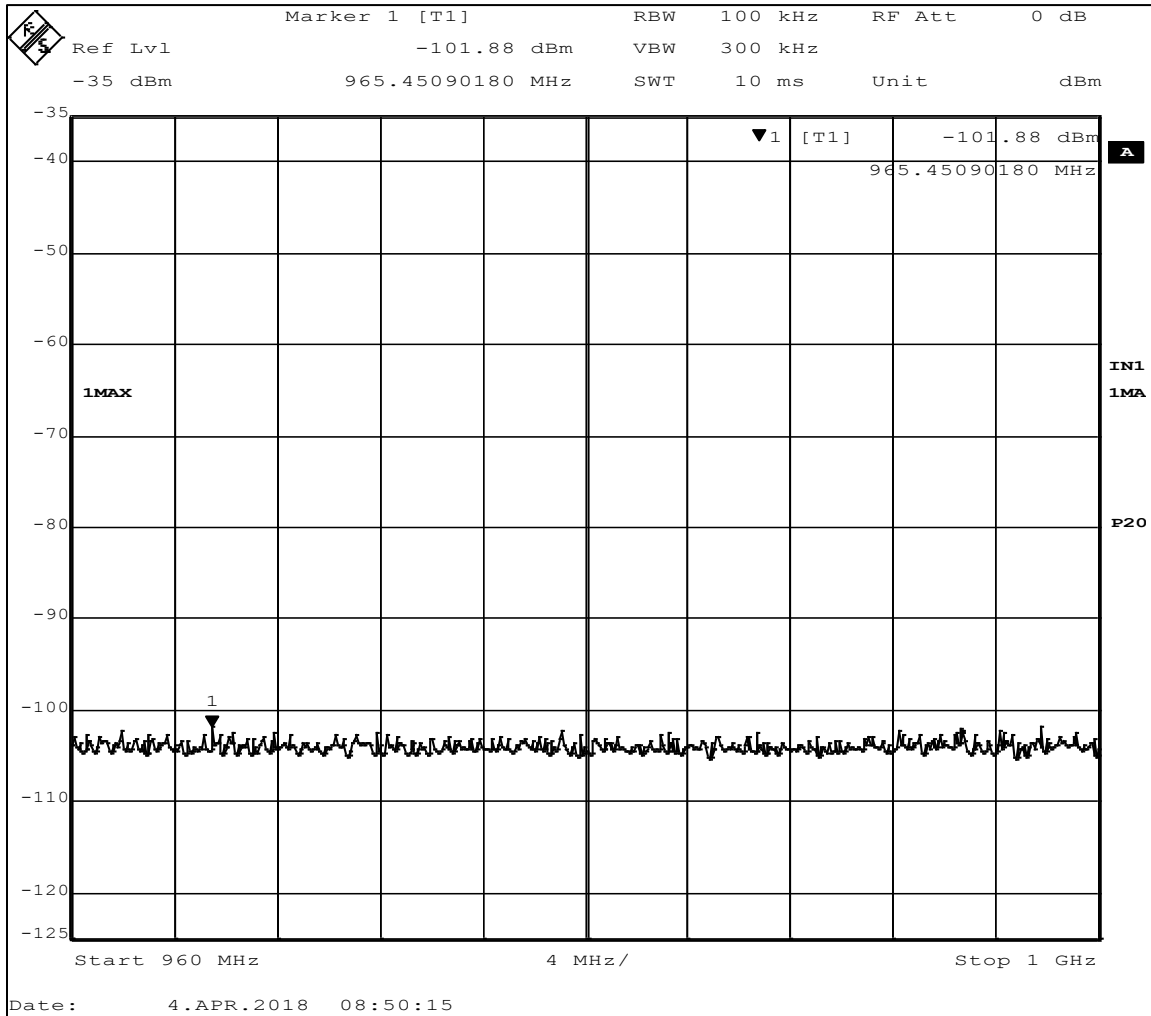
Figure 23 - Band-edge Measurement, High Channel, Restricted Frequency, Hopping The plot shows an uncorrected measurement, used for relative measurements only.
