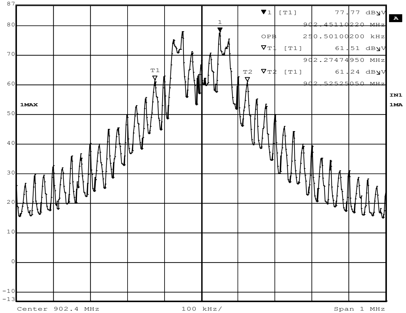
Figure 15 – Occupied Bandwidth, Low Channel. 250.50 kHz
