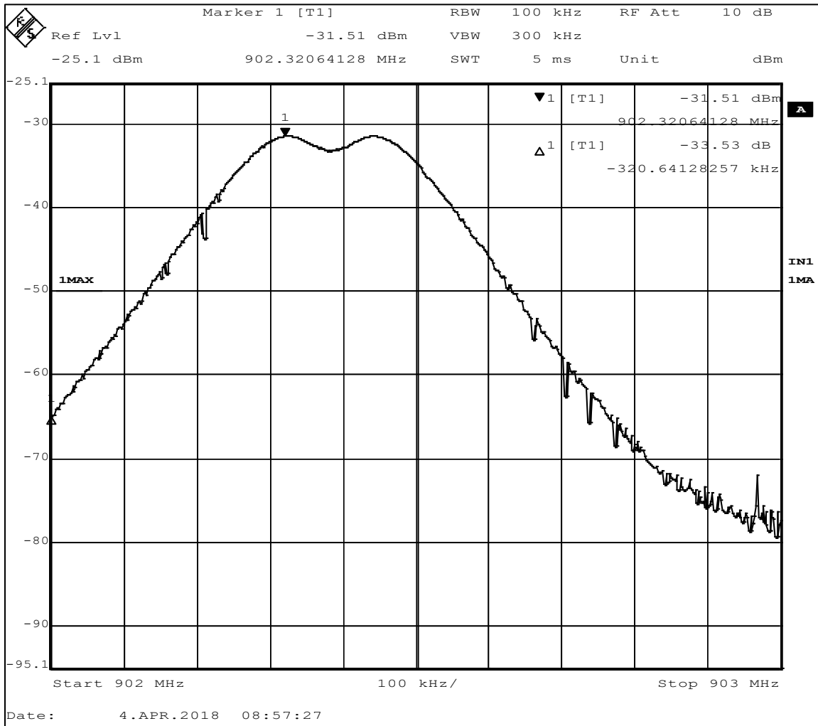
Figure 21 - Band-edge Measurement, Low Channel, Fundamental, Hopping Transmit
