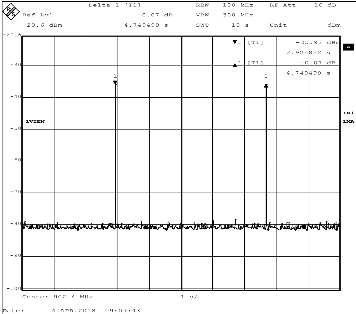
Figure 29 – Time of Occupancy, Period
