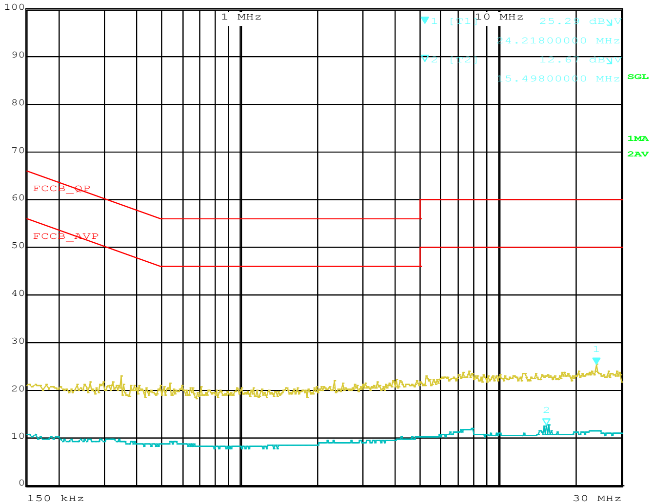
Figure 31 - Conducted Emissions Plot, - Ve Lead
