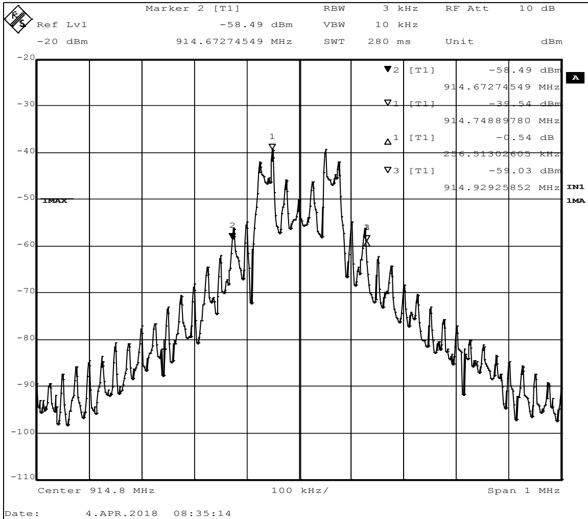
Figure 13 - 20 dB Bandwidth, Mid Channel, 256.51 kHz
