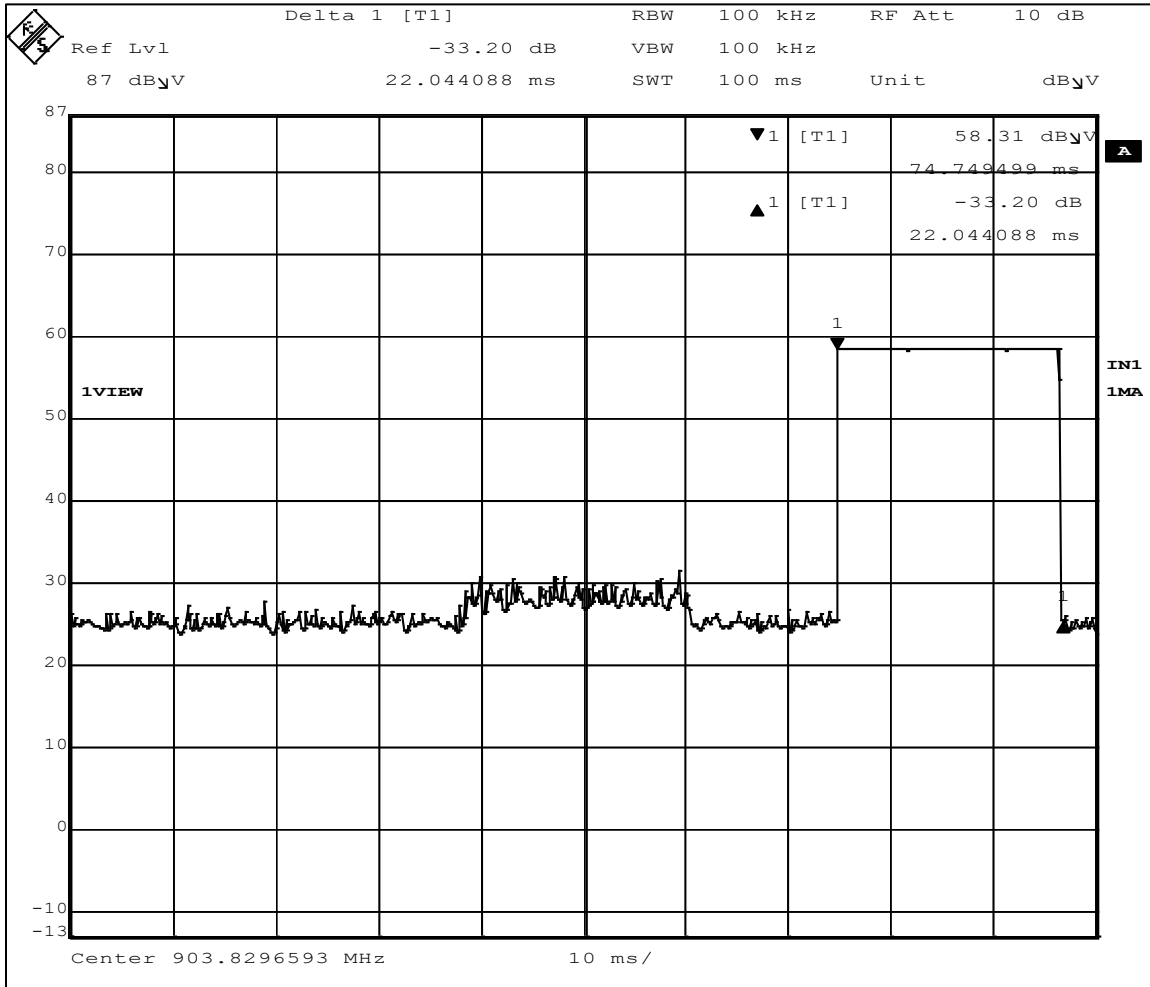
Figure 28 – Time of Occupancy, On Time
