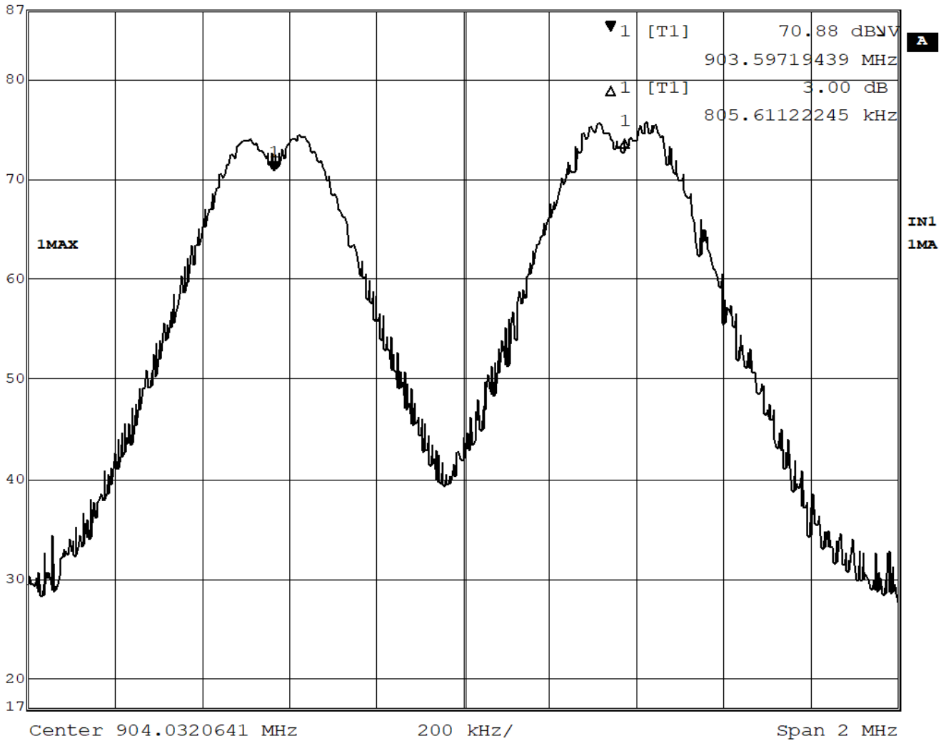
Figure 26 – Frequency Separation, 805.61 kHz
