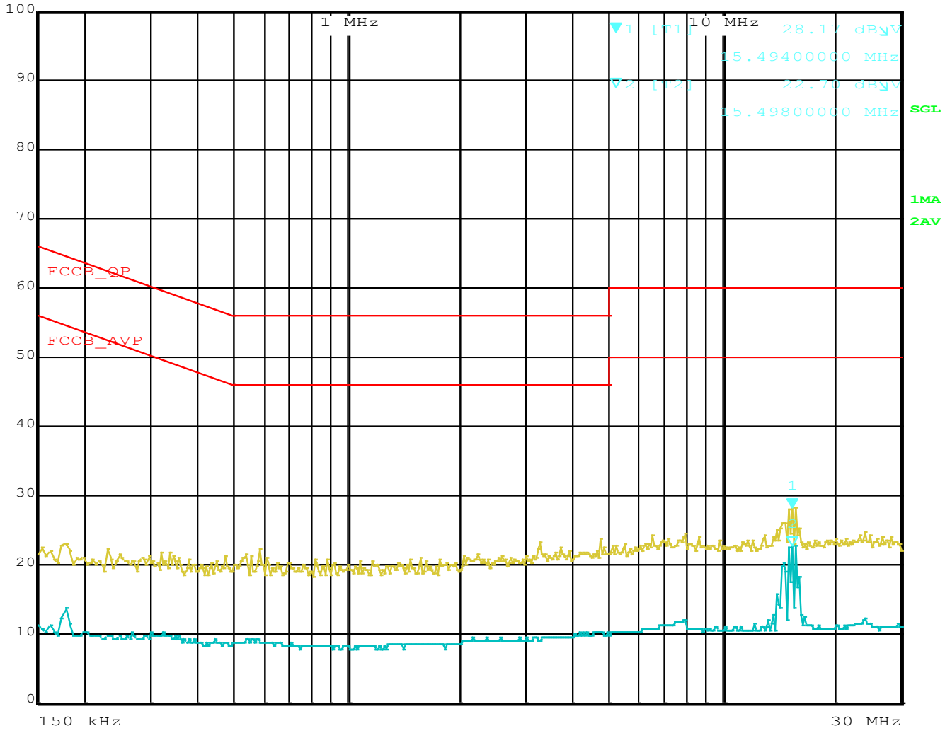
Figure 30 - Conducted Emissions Plot, +Ve Lead
