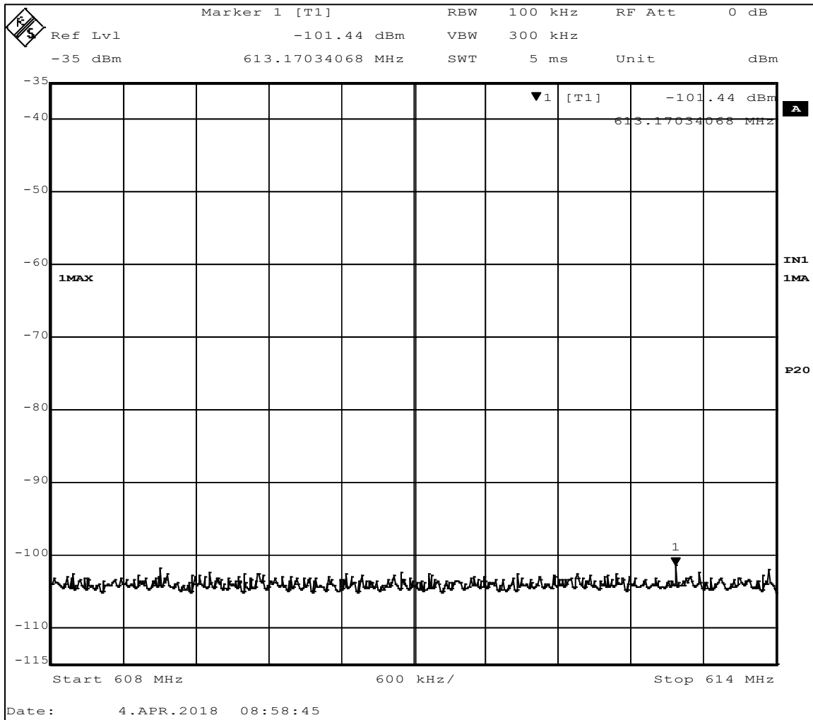
Figure 19 - Band-edge Measurement, Low Channel, Restricted Frequency, Hopping
