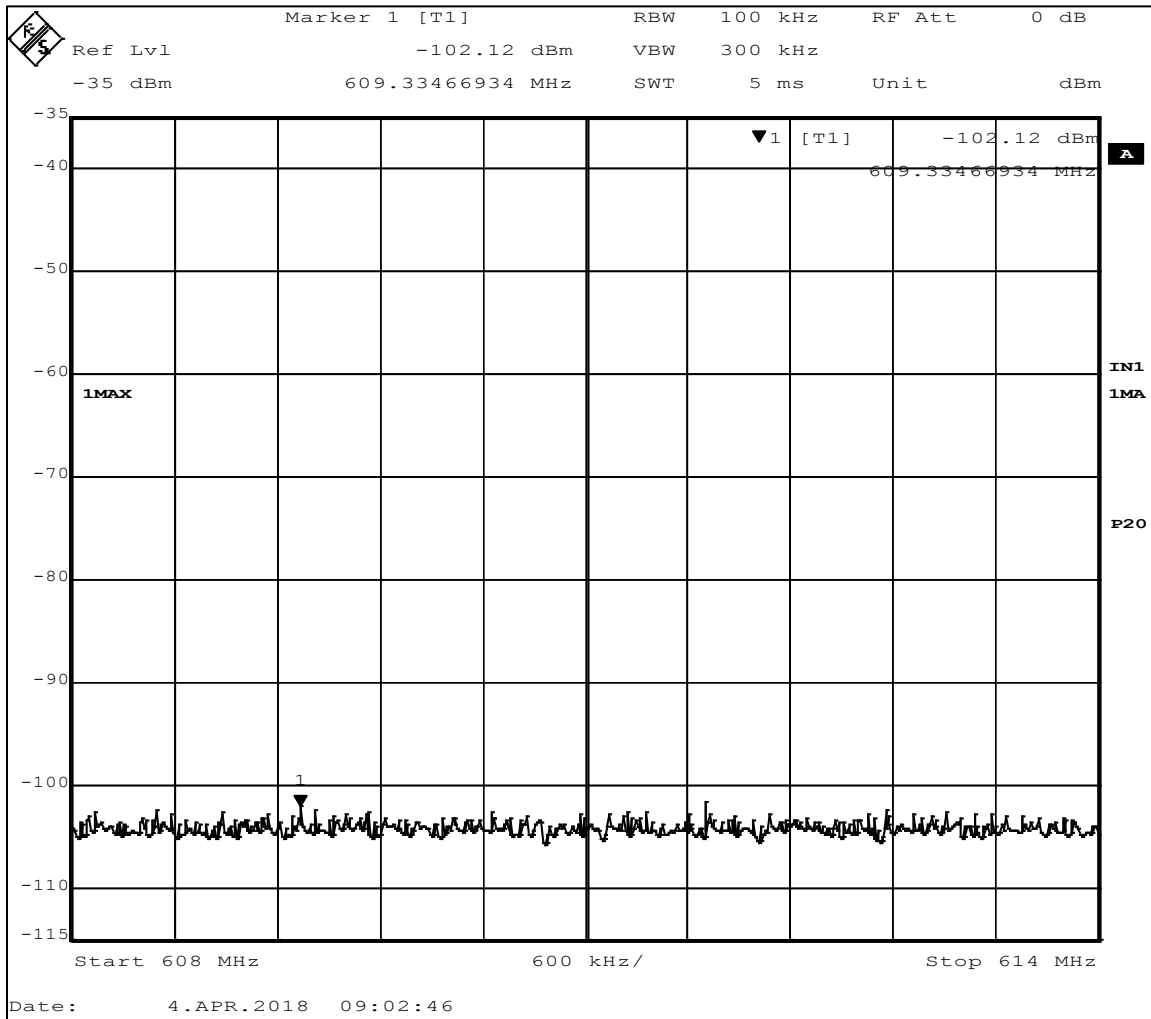
Figure 18 - Band-edge Measurement, Low Channel, Restricted Frequency, Continuous Transmit The plot shows an uncorrected measurement, used for relative measurements only.
