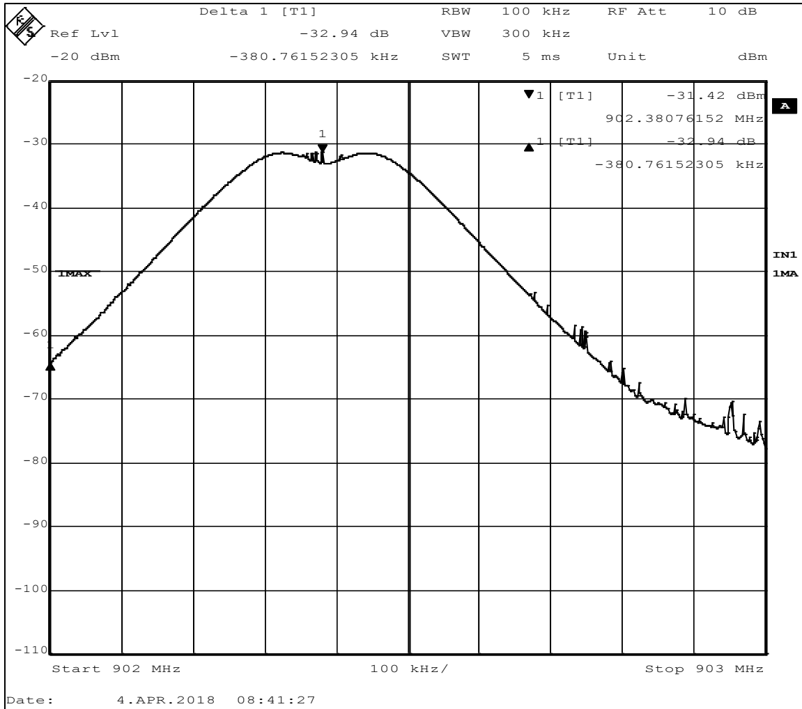
Figure 20 - Band-edge Measurement, Low Channel, Fundamental, Continuous Transmit
