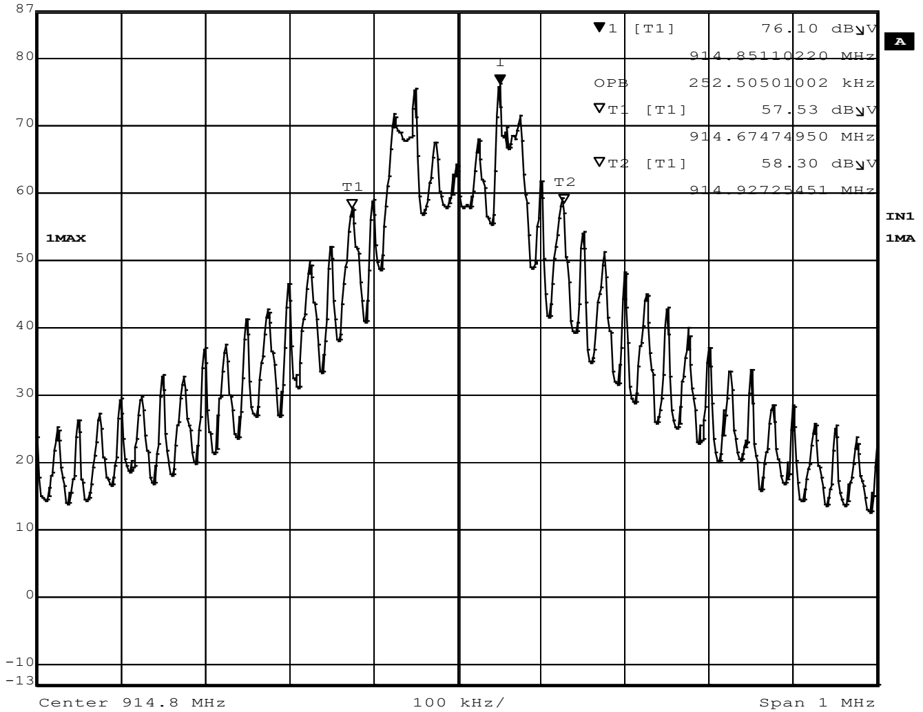
Figure 16 – Occupied Bandwidth, Mid Channel, 252.51 kHz
