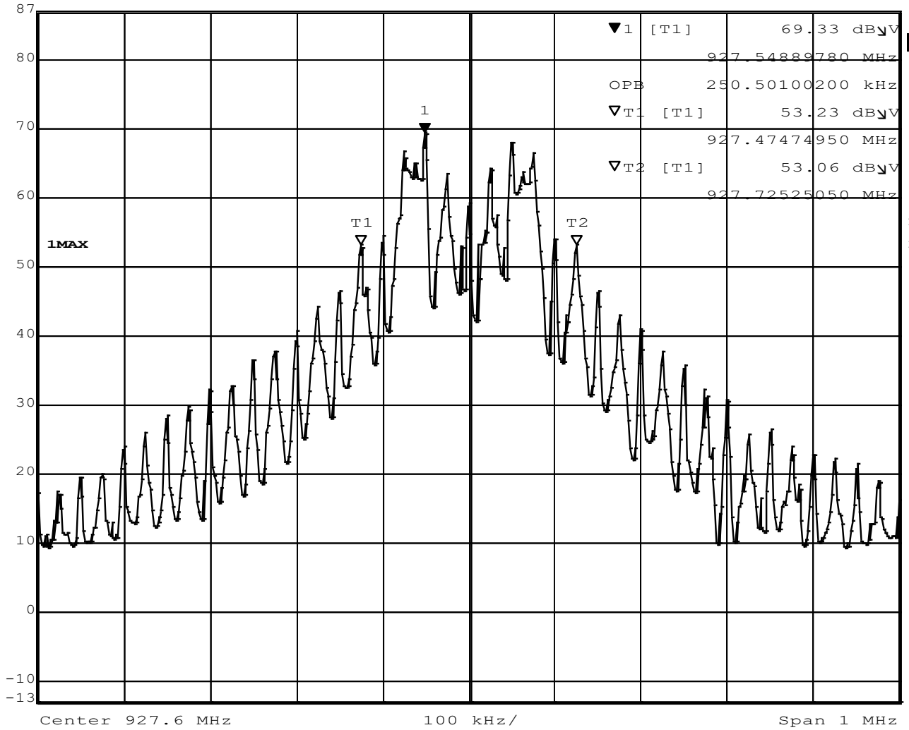
Figure 17 - Occupied Bandwidth, High Channel, 250.50 kHz
