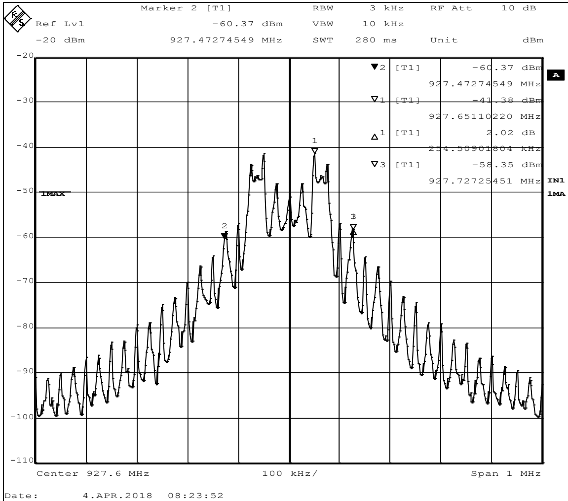
Figure 14 - 20 dB Bandwidth, High Channel, 254.51 kHz
