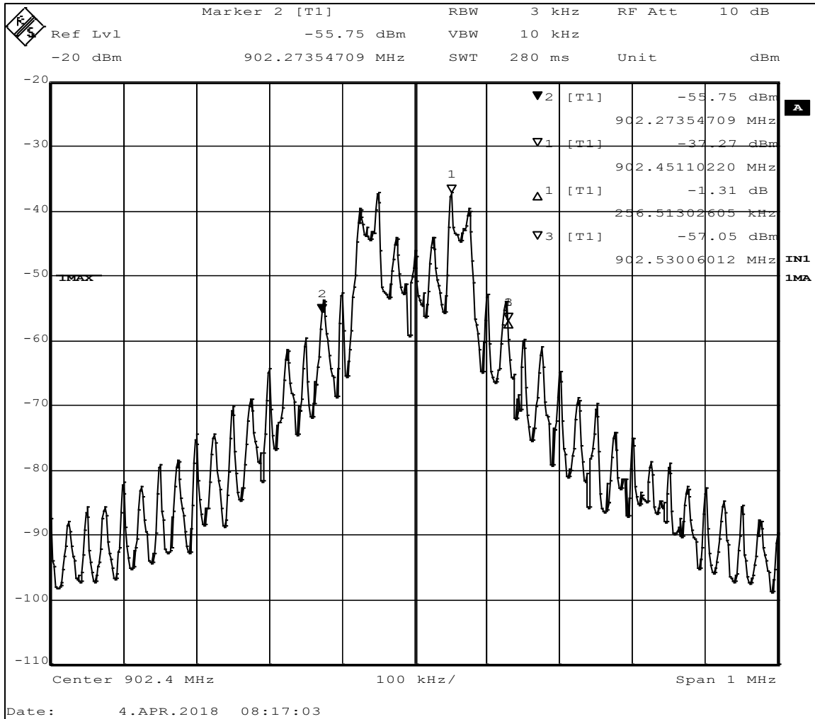
Figure 12 – 20 dB Bandwidth, Low Channel. 256.51 kHz
