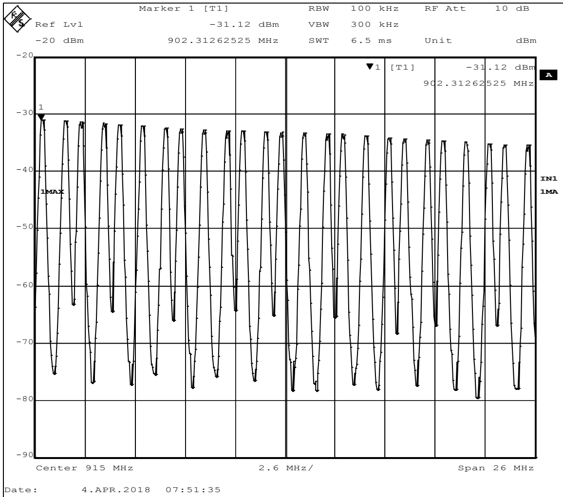
Figure 27 – Hop Count, 25 Hops
