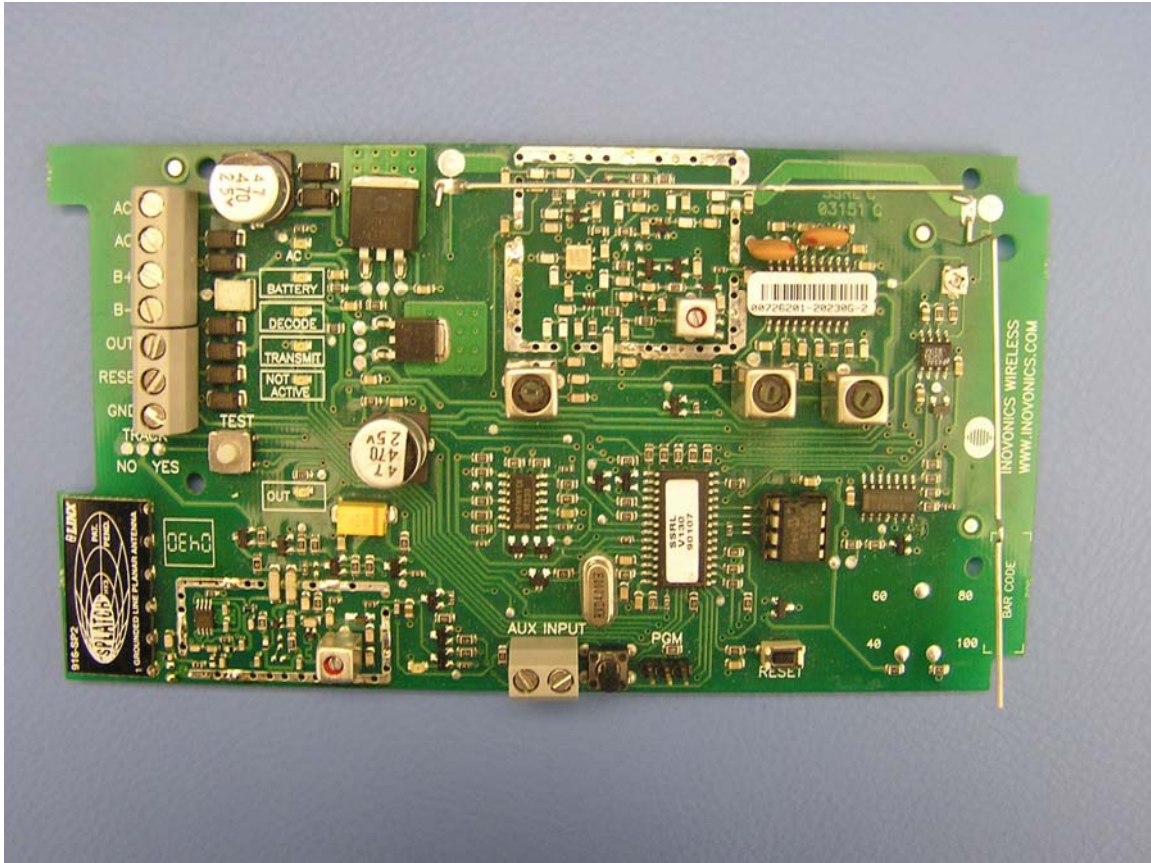
Front PCB with both shield cans removed.
