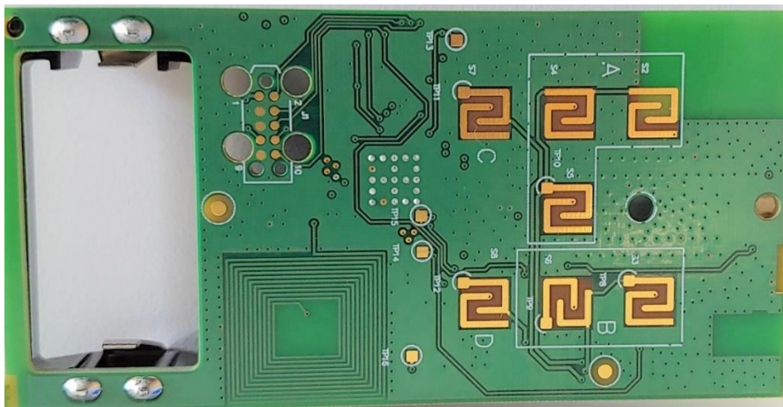
Backside View
