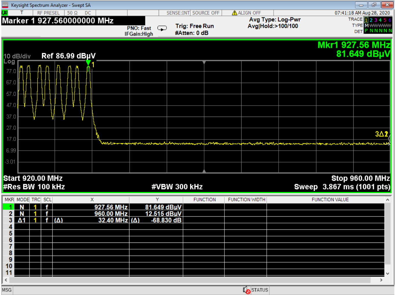
Figure 15 - Band-edge Measurement, High Channel, Fundamental, Hopping Transmit The plot shows an uncorrected measurement, used for relative measurements only. Delta = -68.830 dB > 20 dB Passing unrestricted band edge
