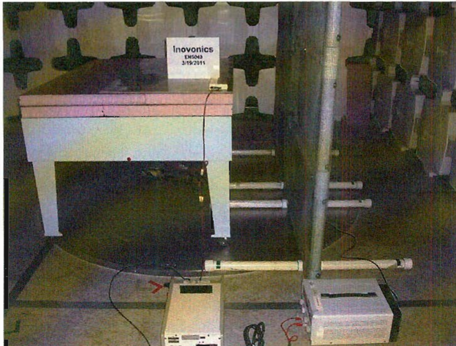
Test setup - Side View (CC1)
