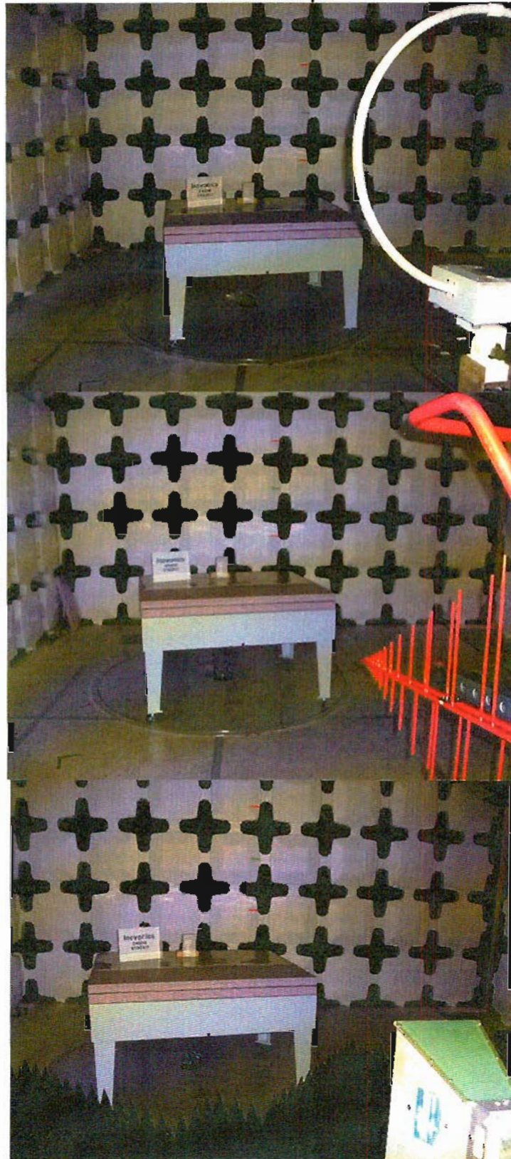
Antenna Setups
