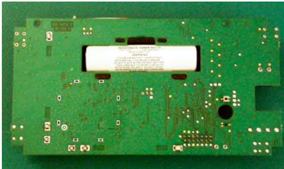
Bottom of PCB
