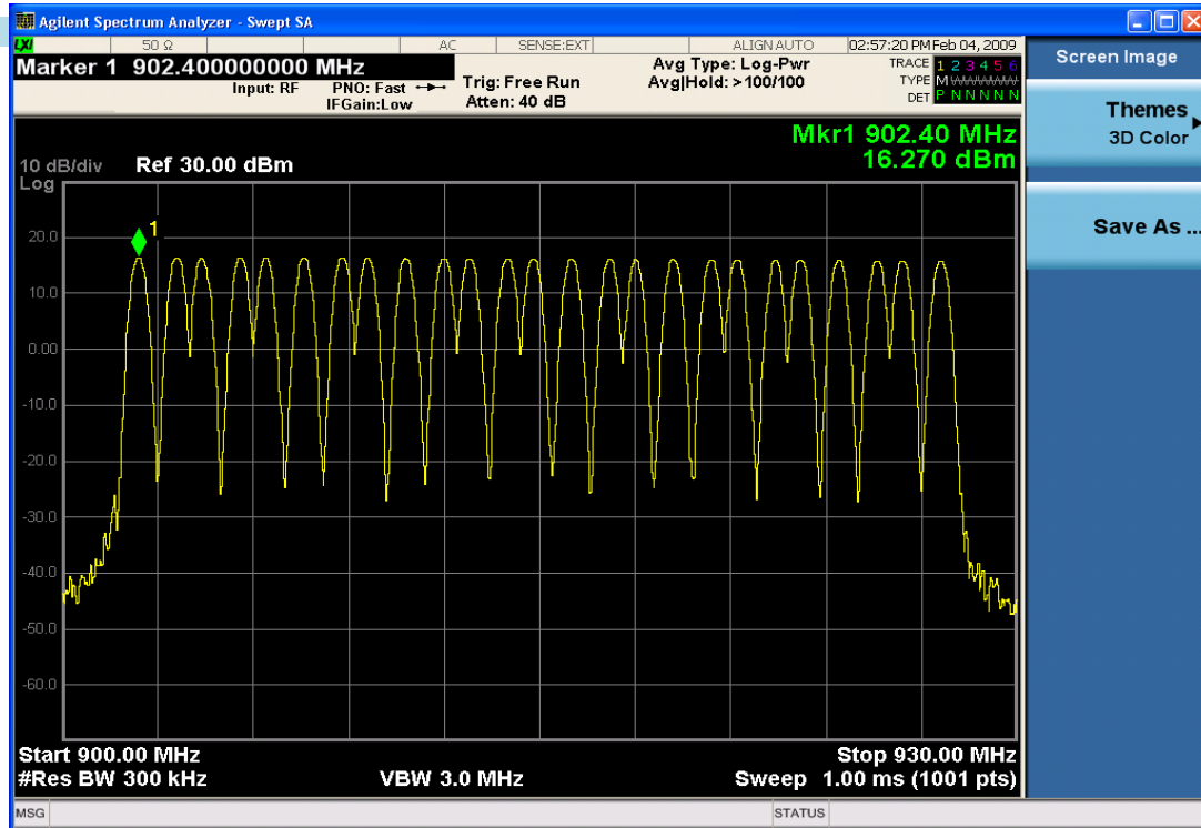
Plot 3: Demonstration of 25 hopping channels.
