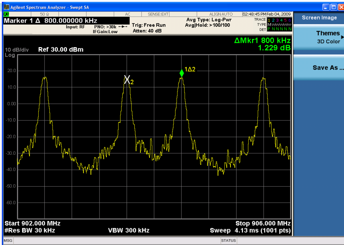
Plot 1: Demonstration of channel spacing requirement.
