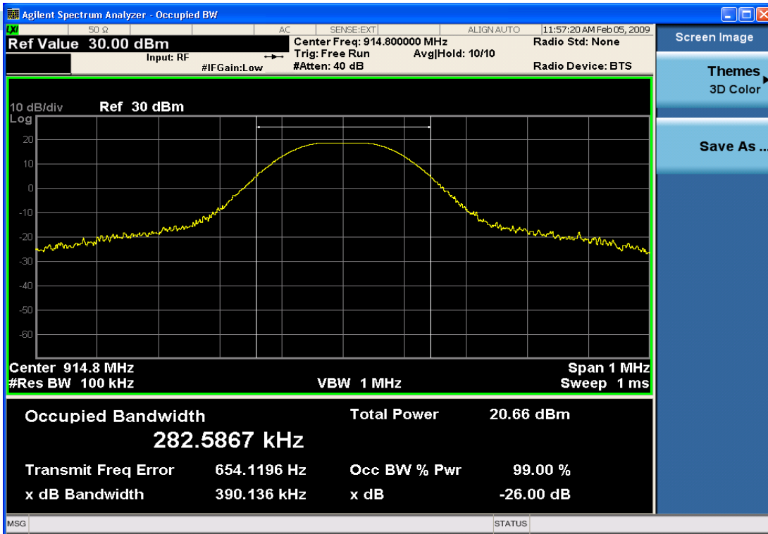
Plot 2: Occupied Bandwidth at lower frequency
