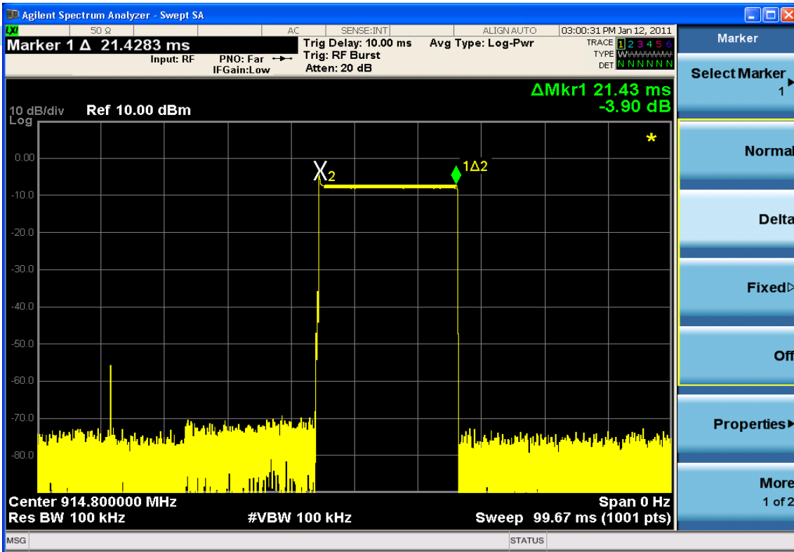
Plot 4: Demonstration of Frequency Dwell Time.
