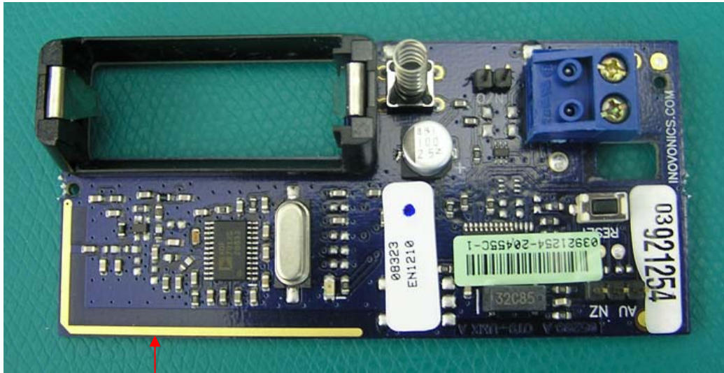
Trace Antenna
