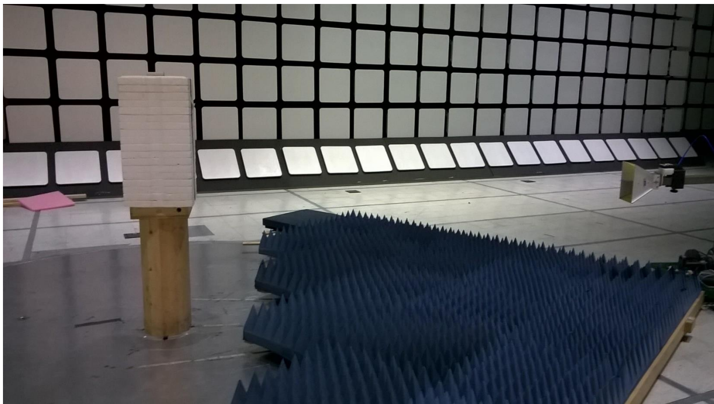
Figure 4 - Radiated Emissions Test Setup, 1 - 25 GHz
