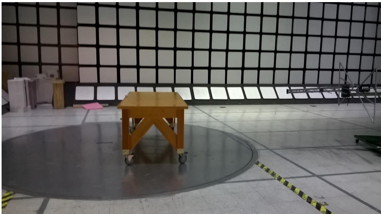
Figure 8 - Test Setup Photos, 30MHz - 1GHz
