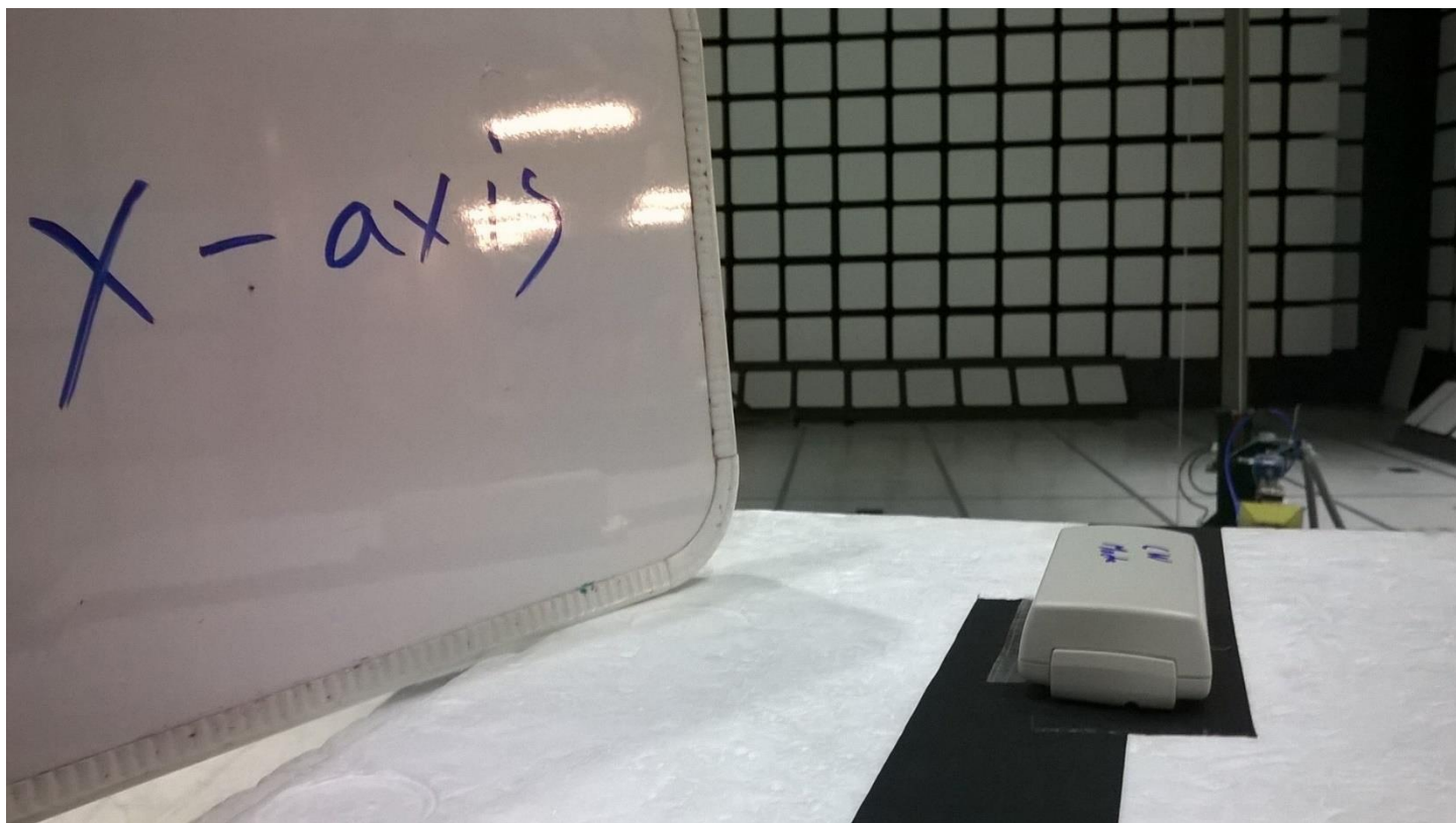
Figure 1 - Radiated Emissions Test Setup, 1 - 25 GHz, x-axis
