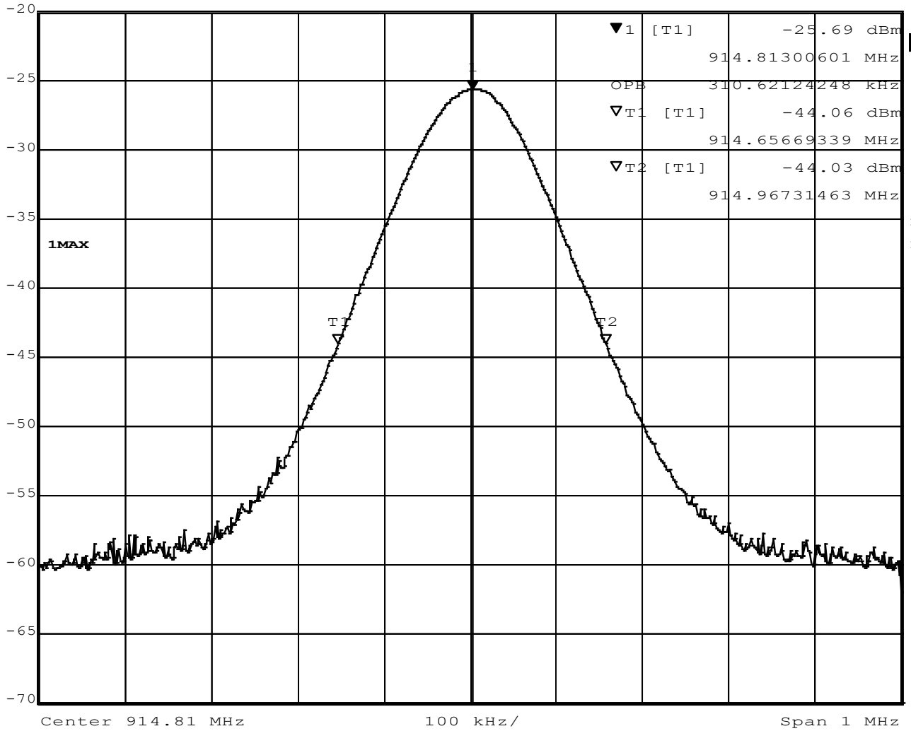
Figure 13 - Occupied Bandwidth, Mid Channel
