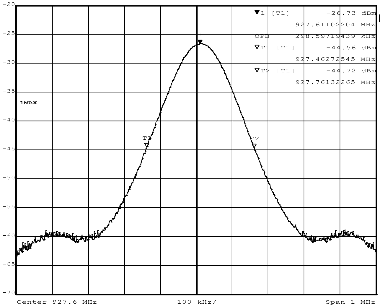
Figure 14 - Occupied Bandwidth, High Channel
