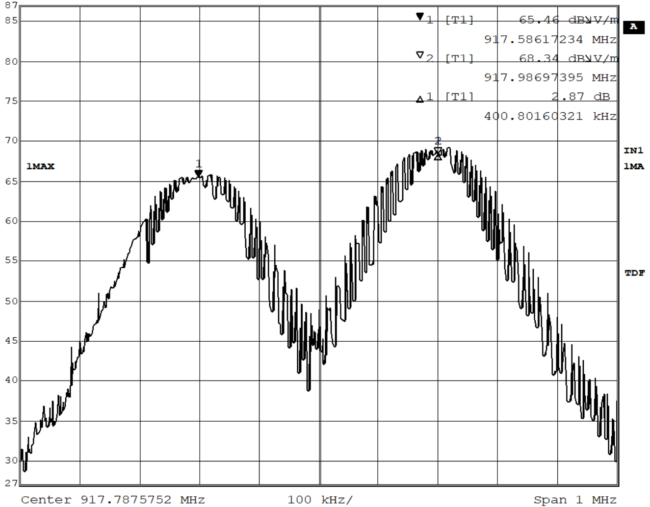
Figure 23 – Frequency Separation
