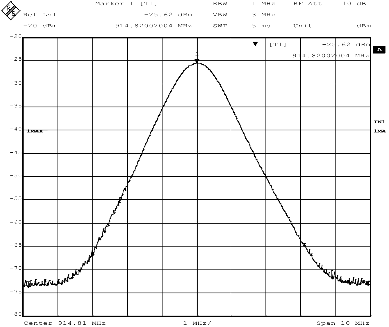
Figure 6 - Output Power, Mid Channel
