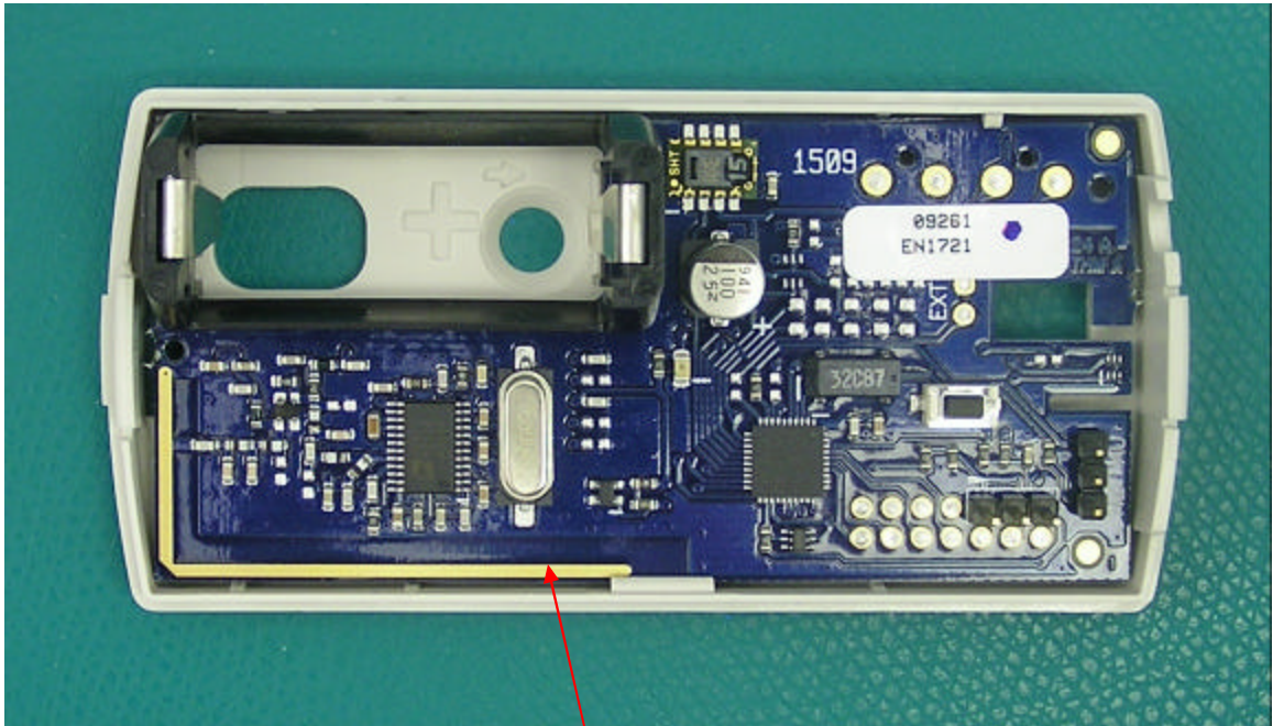
PCB FRONT
