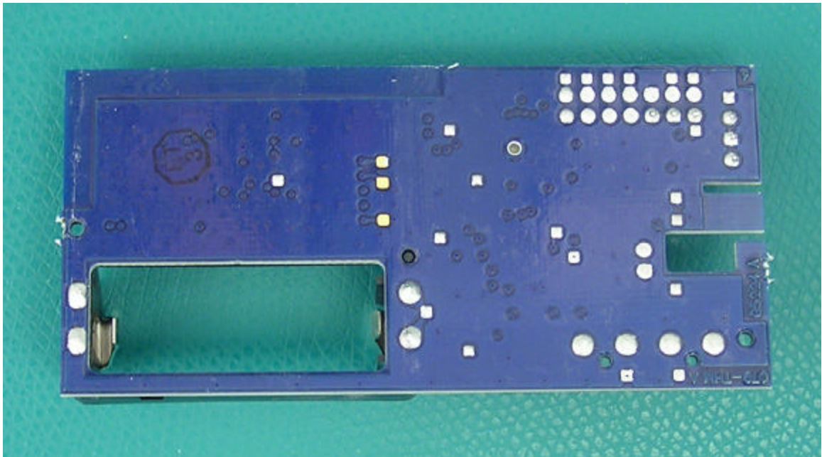
PCB Back
