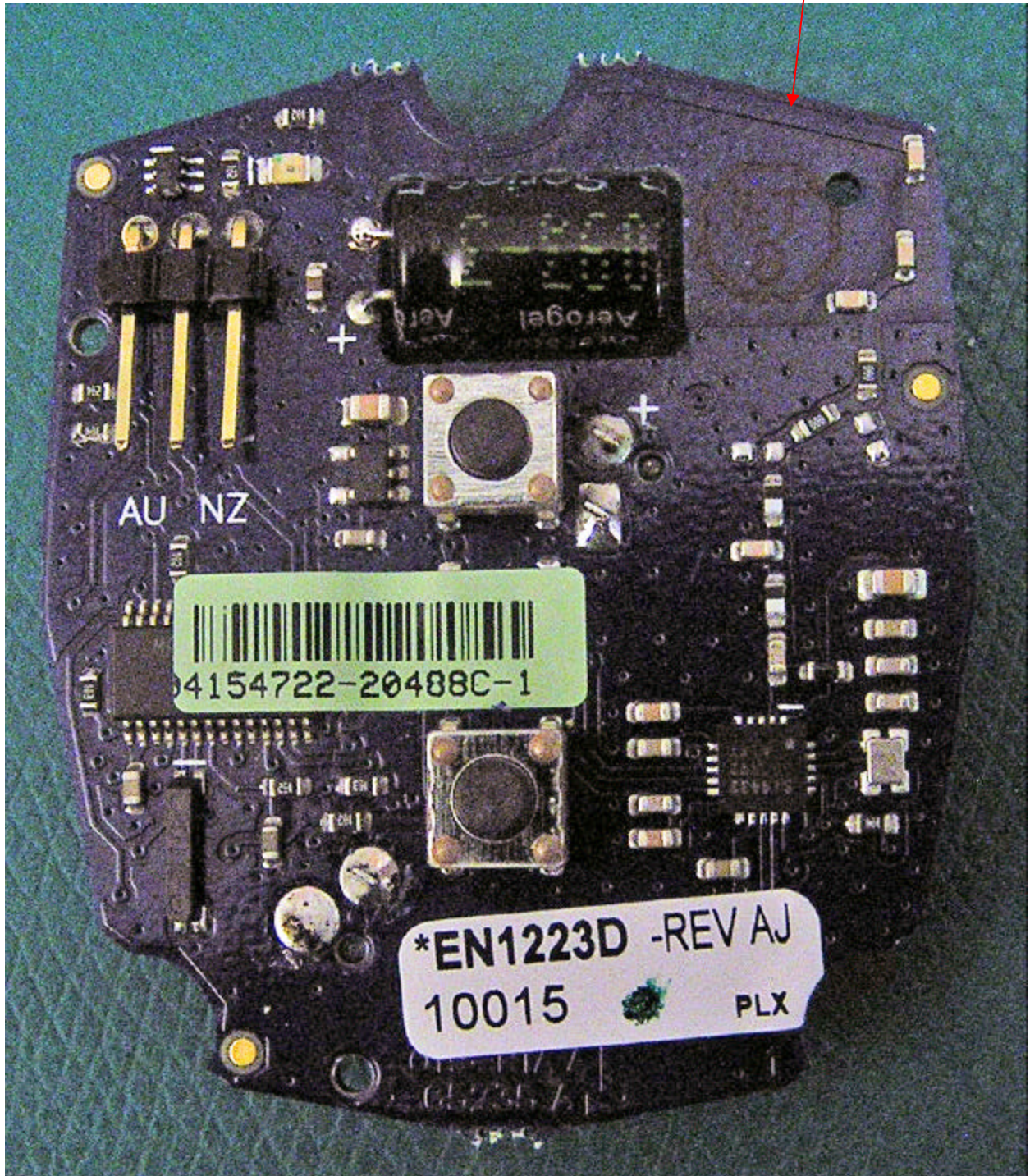
PCB FRONT
