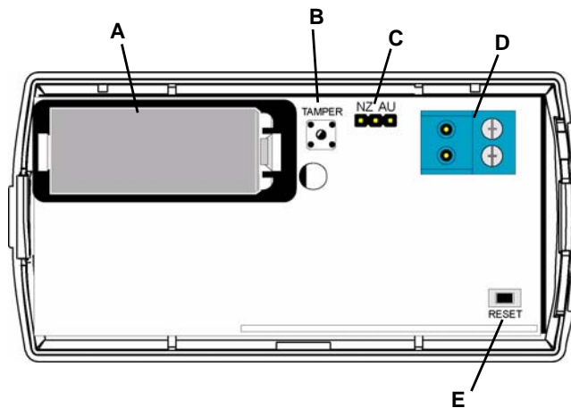
Figure 1 EN1501/EN1501-XL Components
