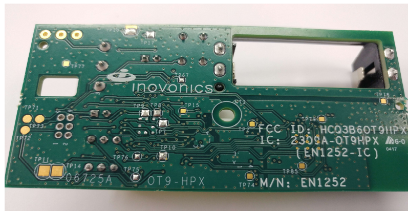
Picture 3 - EN1252 Rear View
