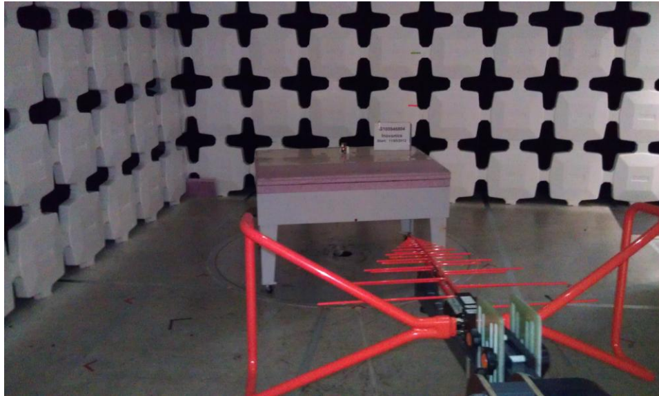
Picture 1 - EMC Chamber Setup
