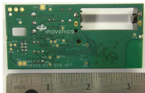
Picture 3 - EN1252 Rear View
