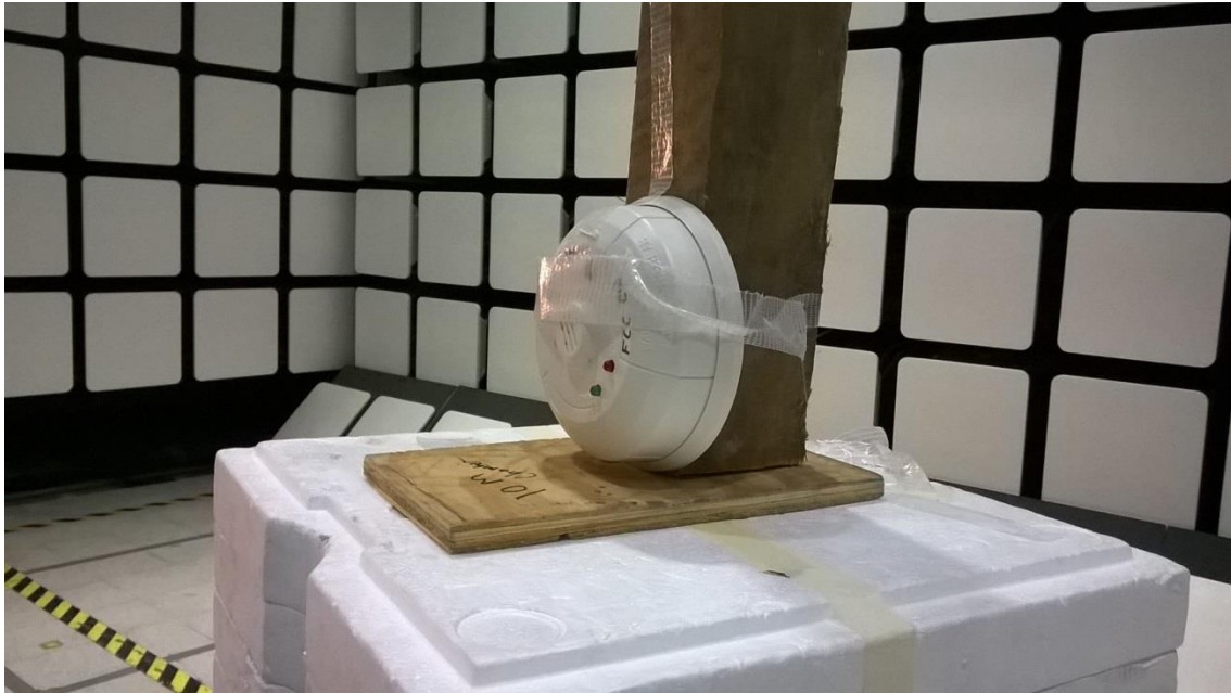
Figure 3 - Radiated Emissions Test Setup, X-axis
