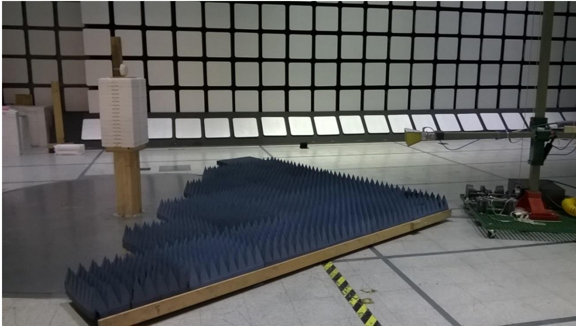
Figure 1 - Radiated Emissions Test Setup, 1 - 10 GHz
