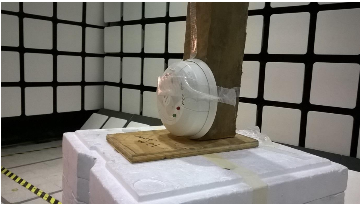
Figure 6 - Radiated Emissions Test Setup,
