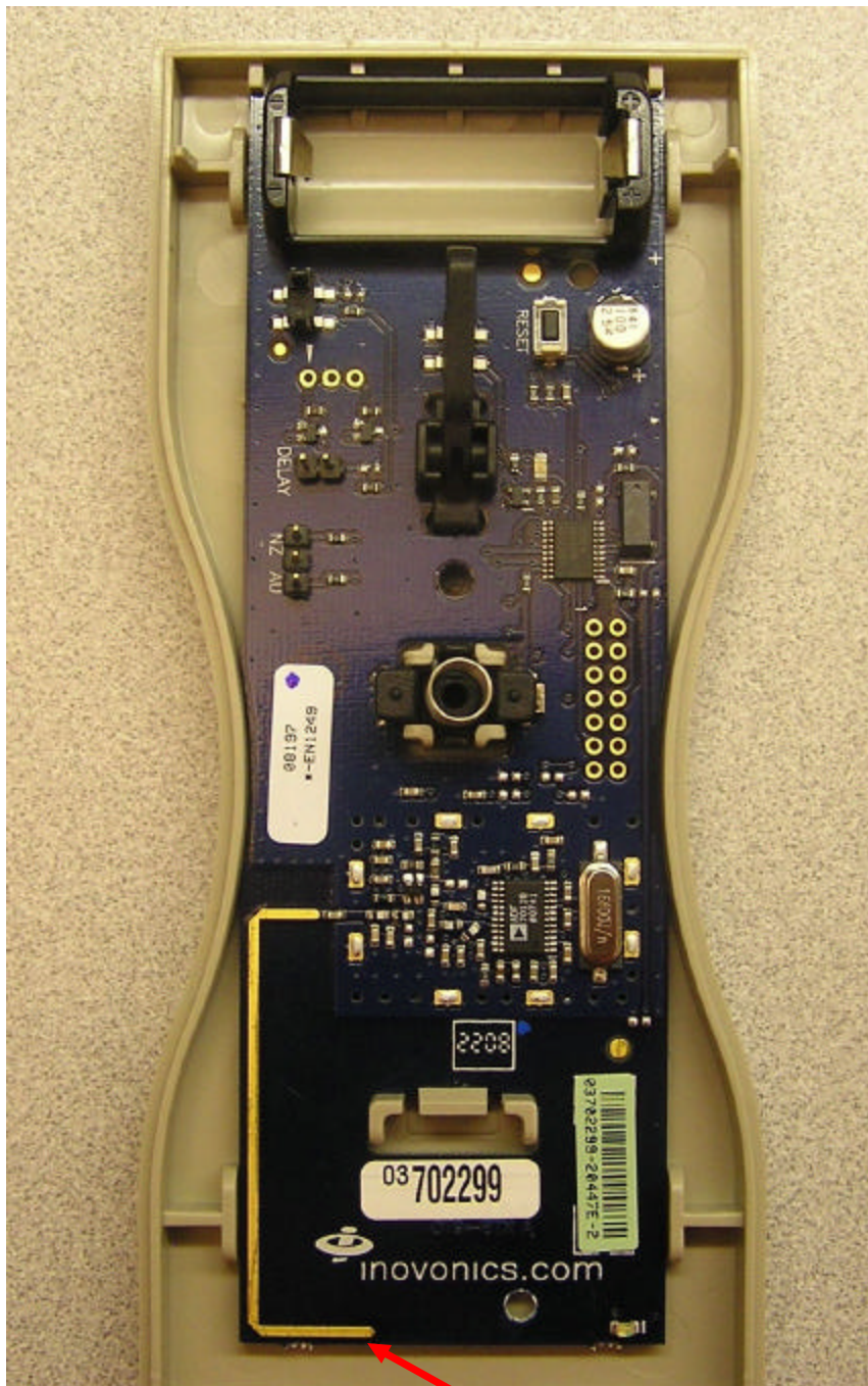
PCB FRONT
