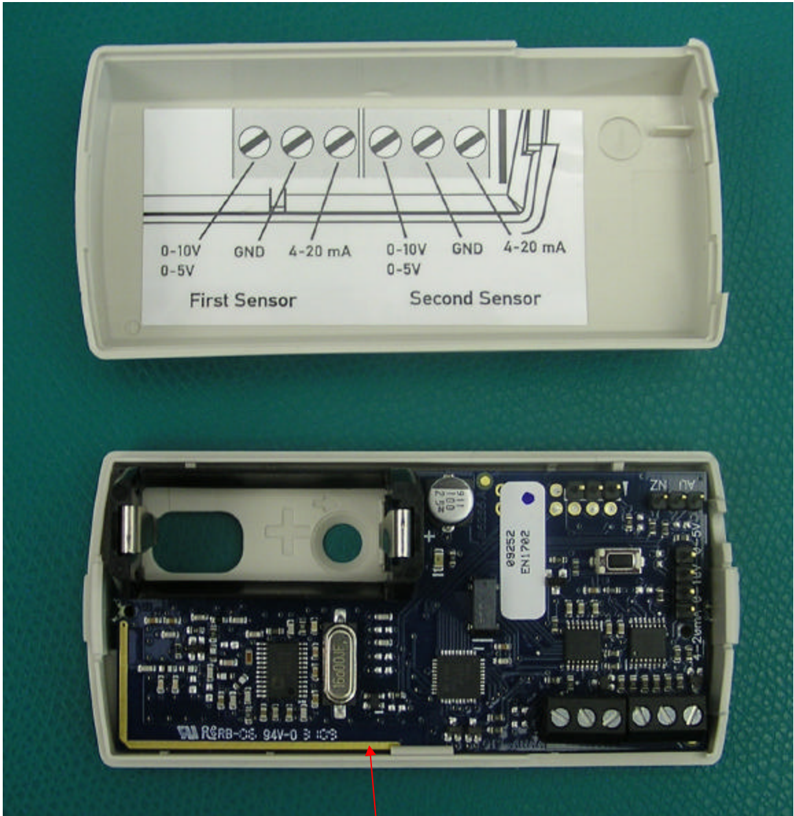
Trace Antenna
