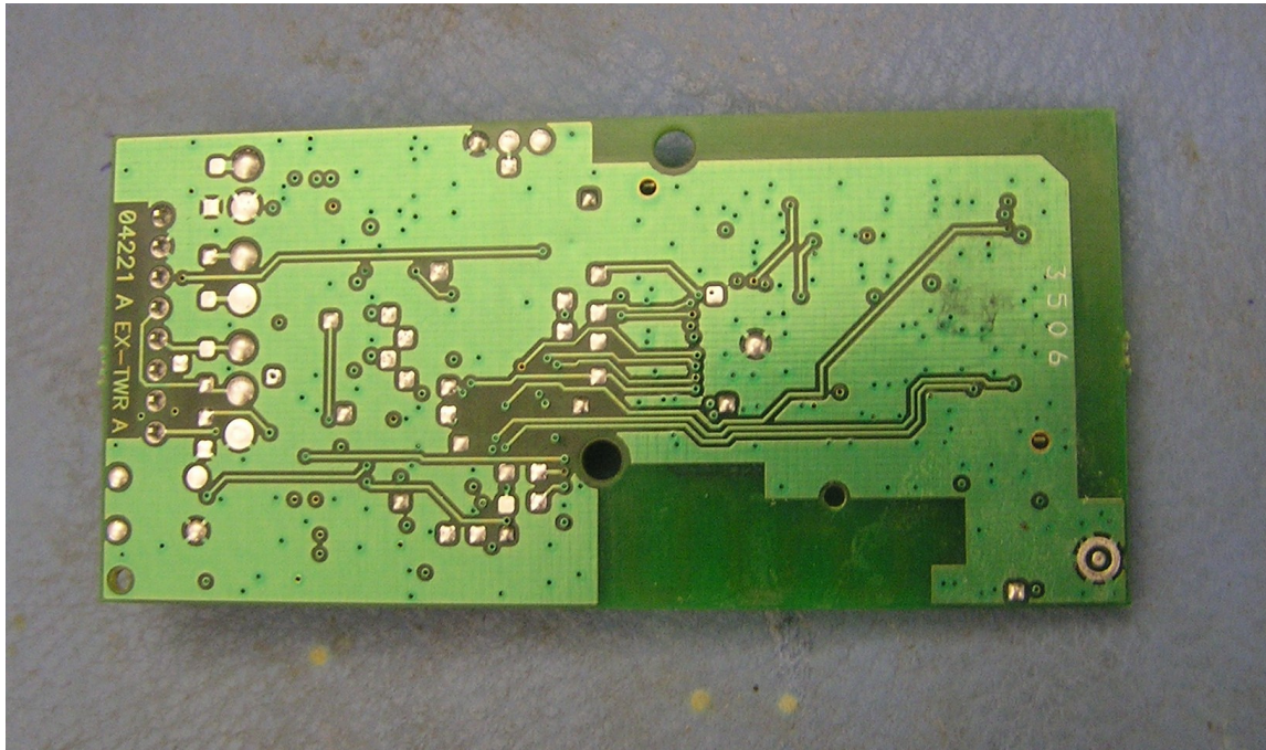
PCB Back
