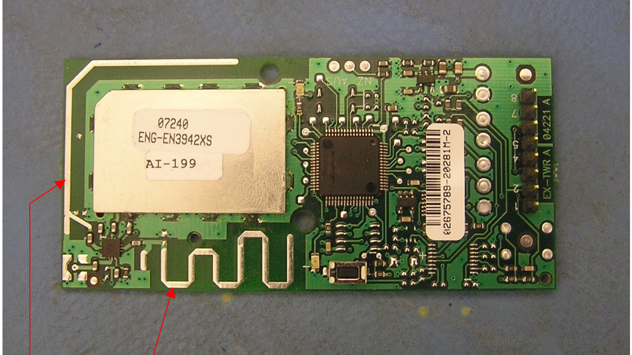
PCB Trace Antenna
