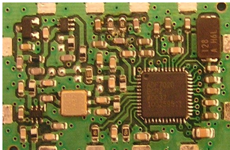
PCB Front Under Shield Can
