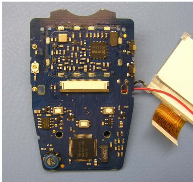
Front of PCB with LCD and RF shielding removed
