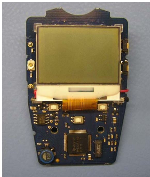
Front of PCB showing LCD Graphics Display
