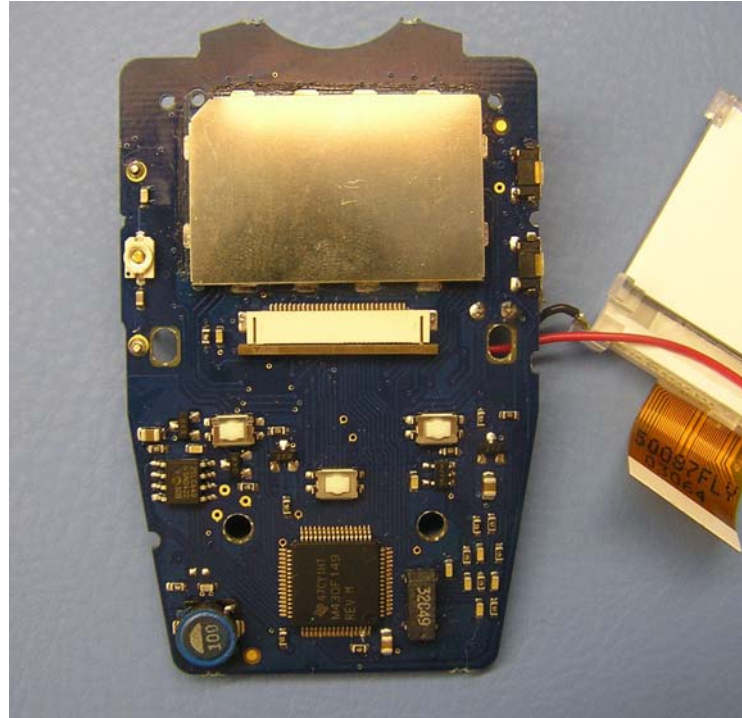
Front of PCB with LCD Graphics Display removed
