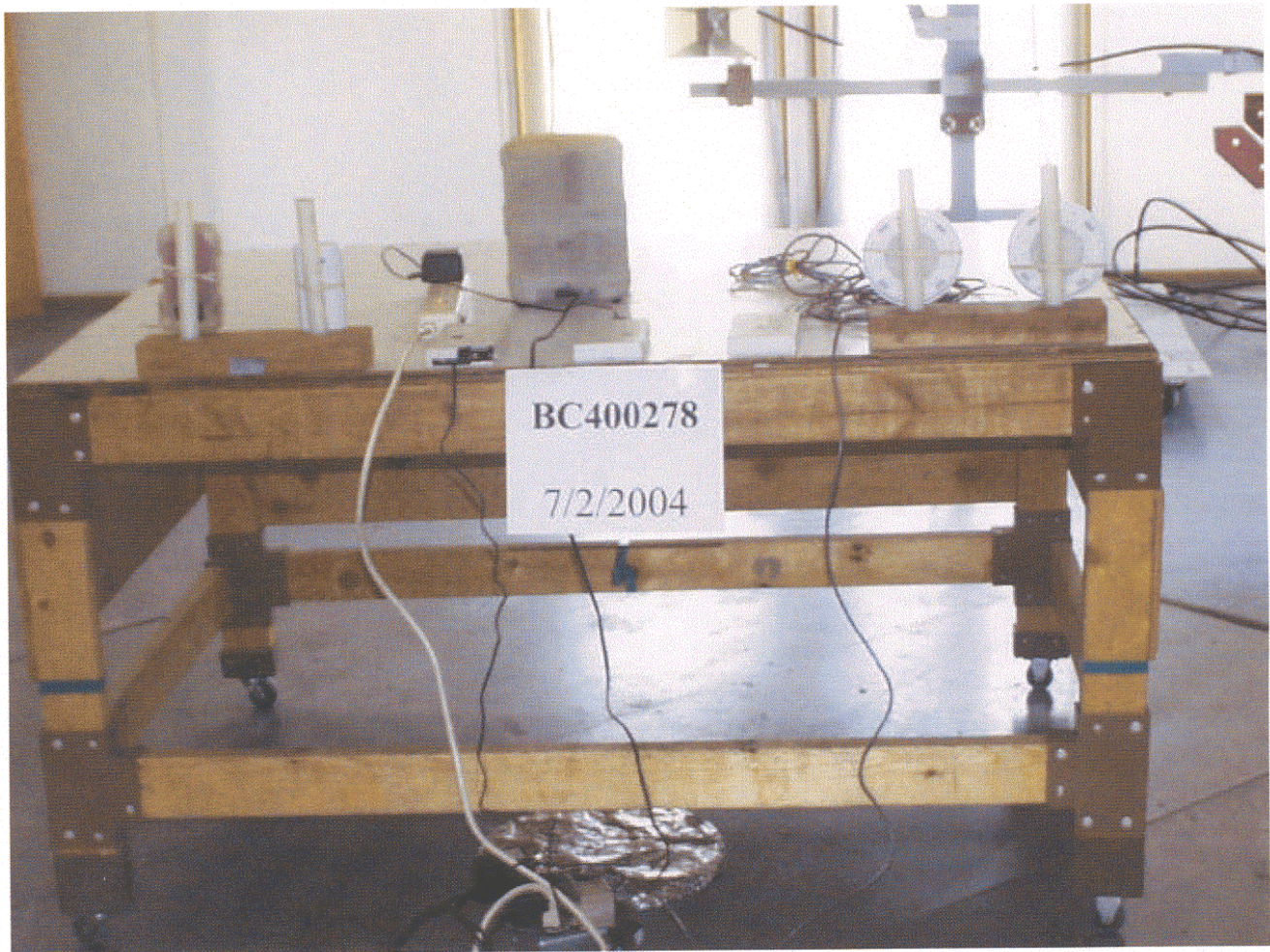
Test-setup photo(s): Radiated Unintentional Emissions
