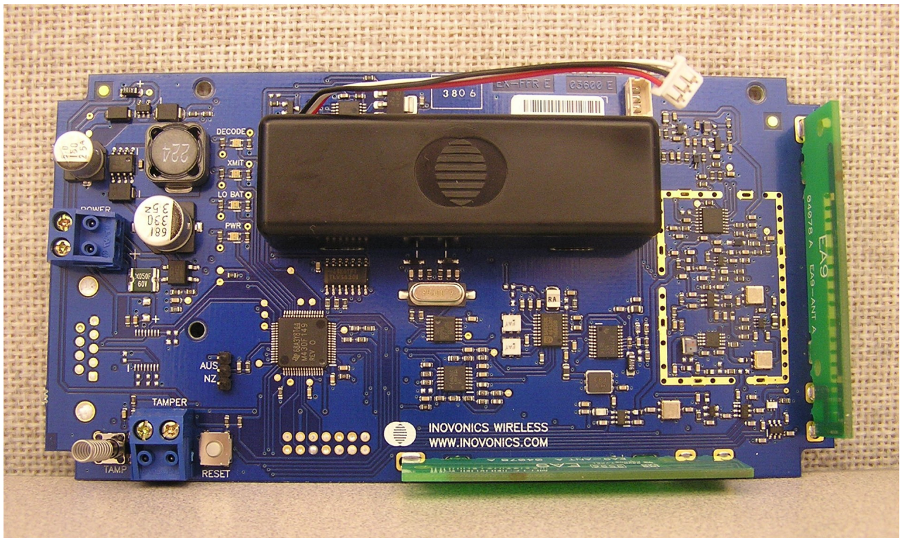
PCB front side, without shield can
