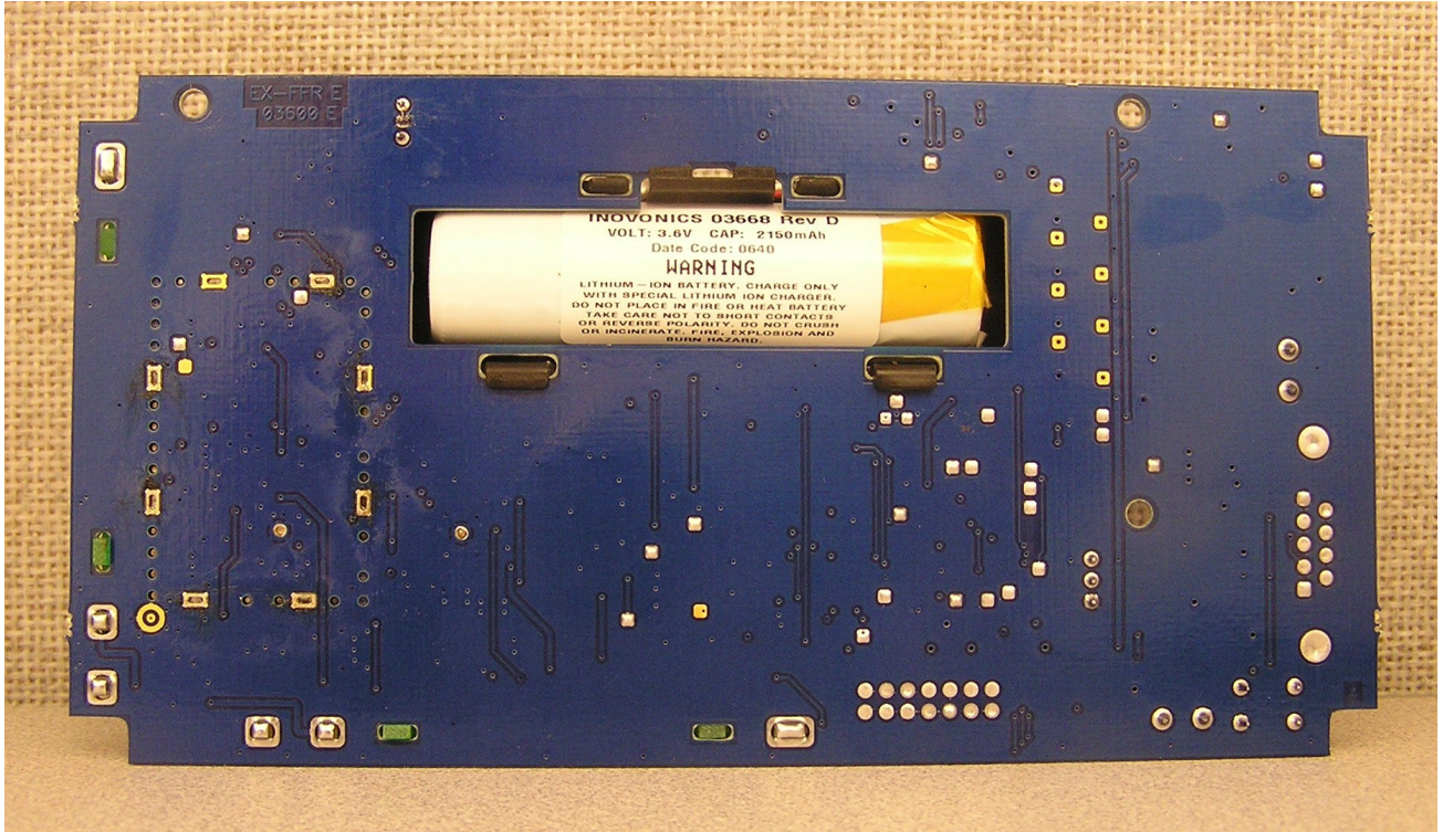
PCB back side
