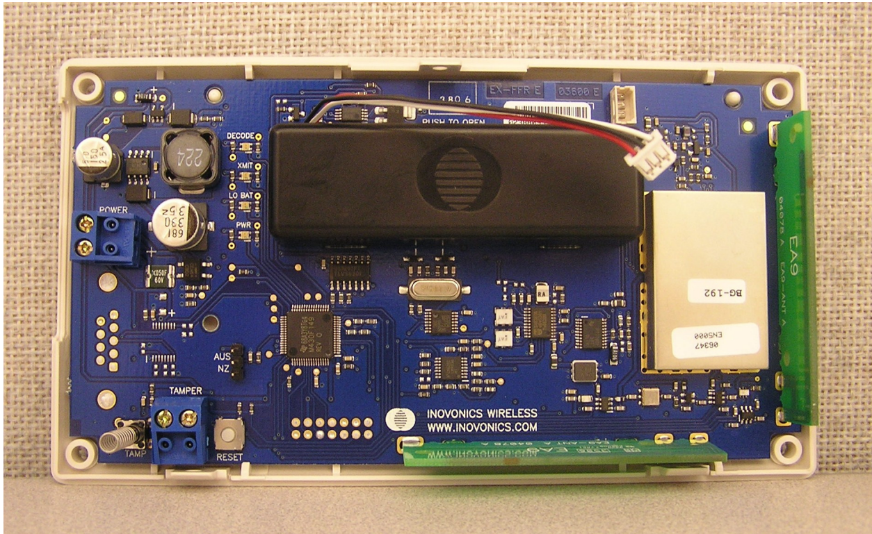
PCB front side, with shield can
