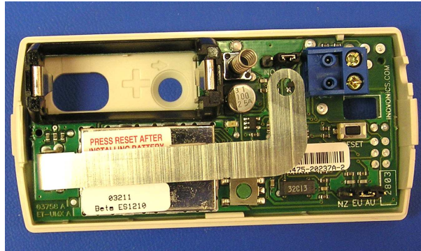
PCB Topside
