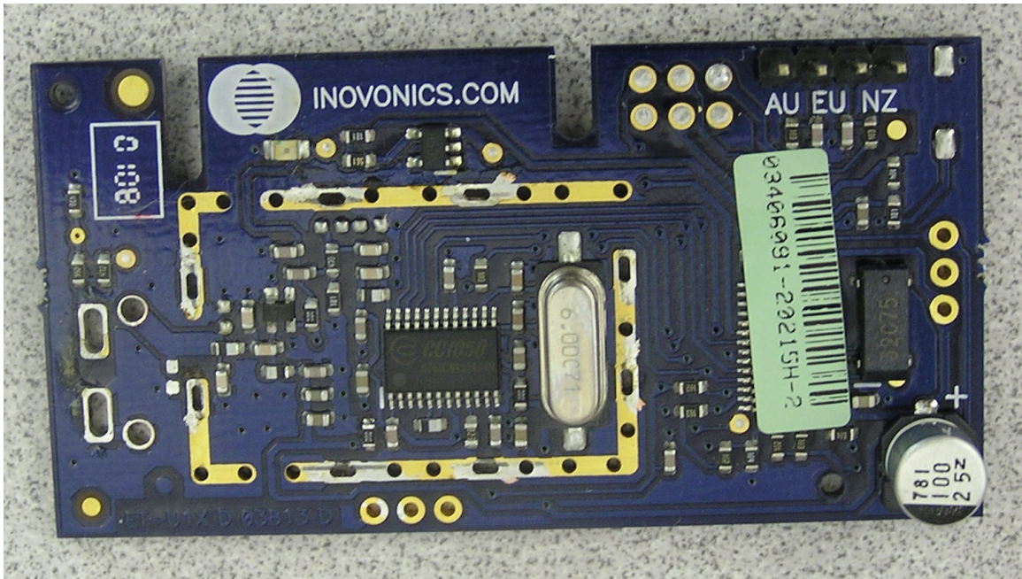
PCB without shield can
