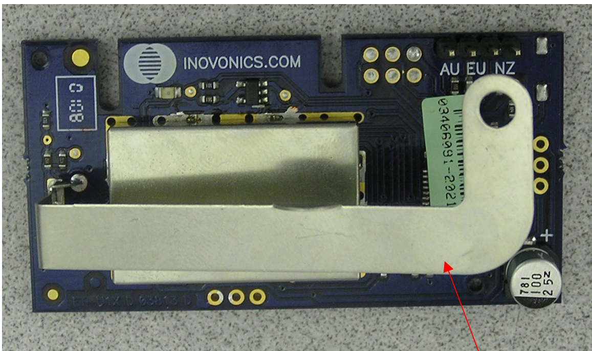
PCB with shield can
