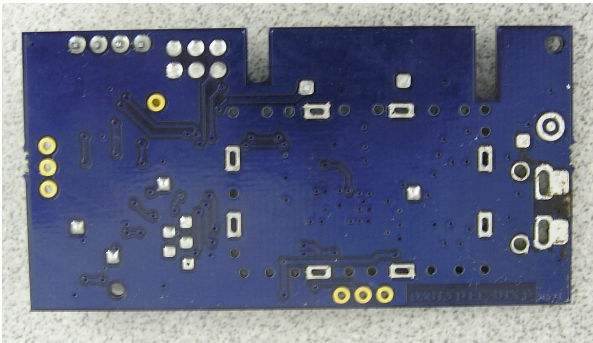
PCB back
