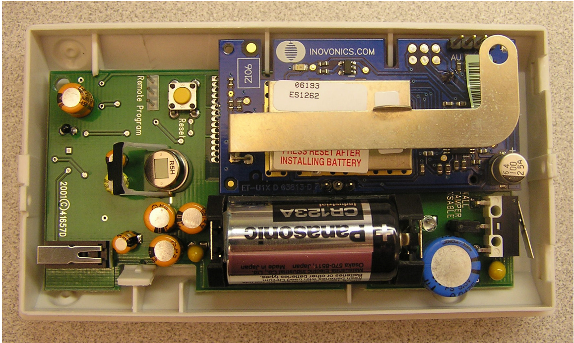
Inside of Unit, without housing
