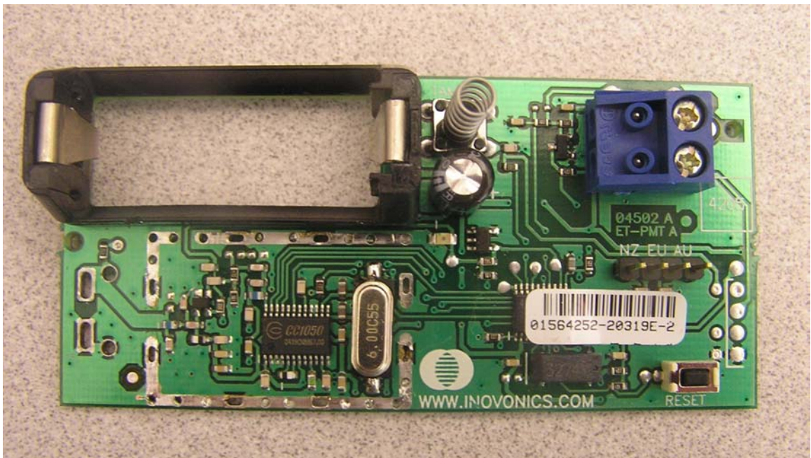
PCB front side, without shield can and antenna
