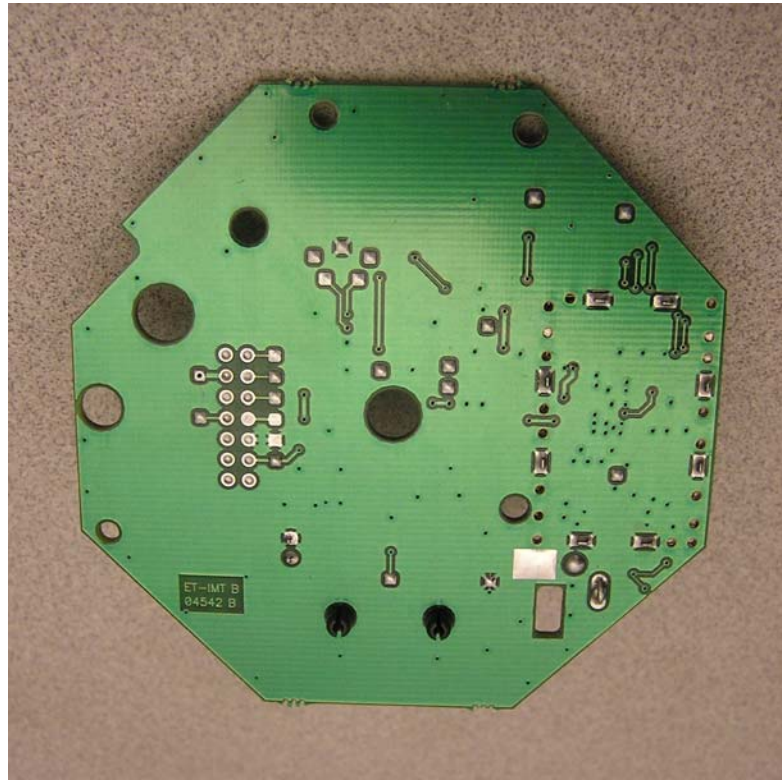
PCB Back
