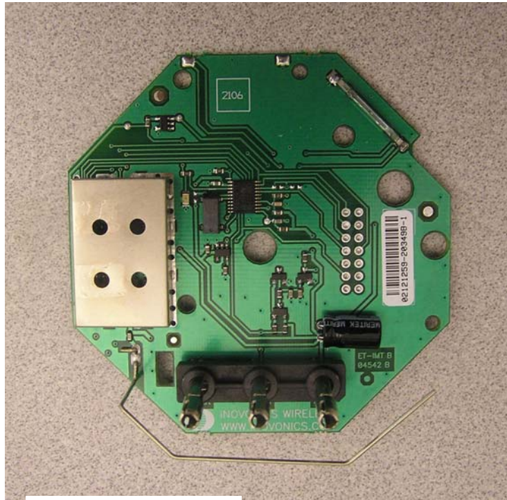
PCB Front
