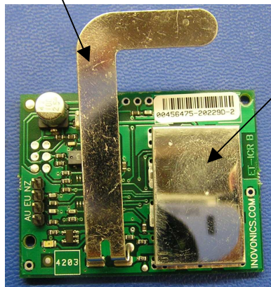
PCB topside
