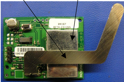
PCB topside
