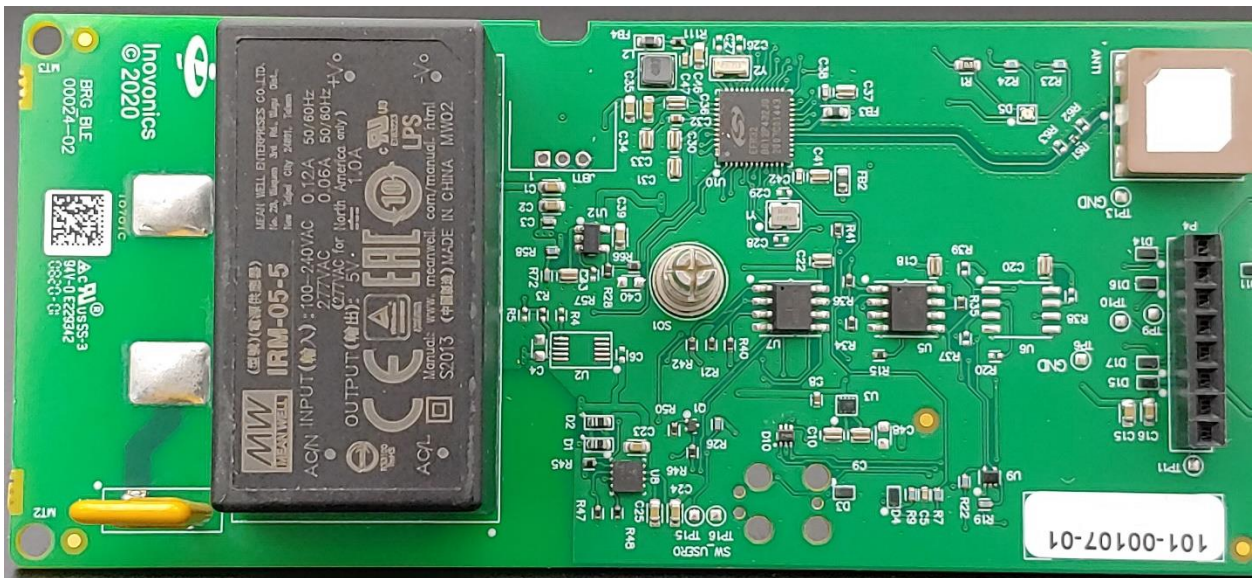
Top View – Main Carrier Printed Circuit Assembly
