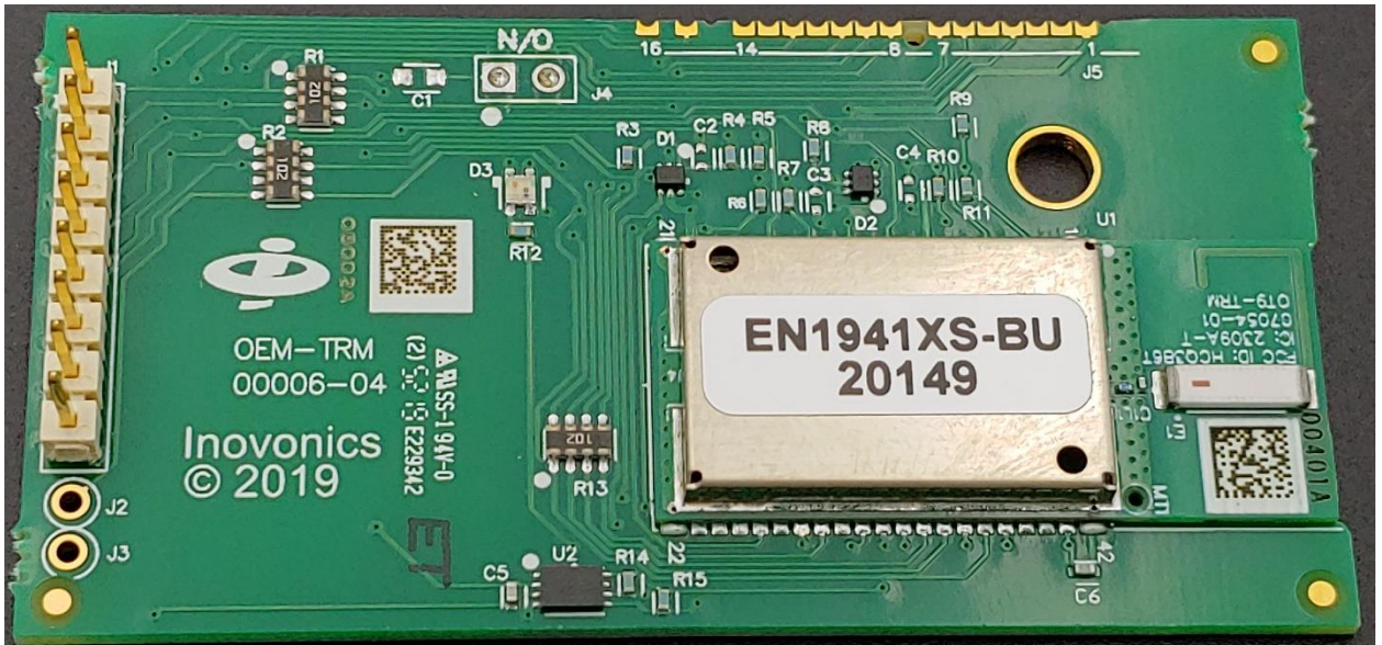
Top View – EN1941XS EchoStream Transmitter Board
