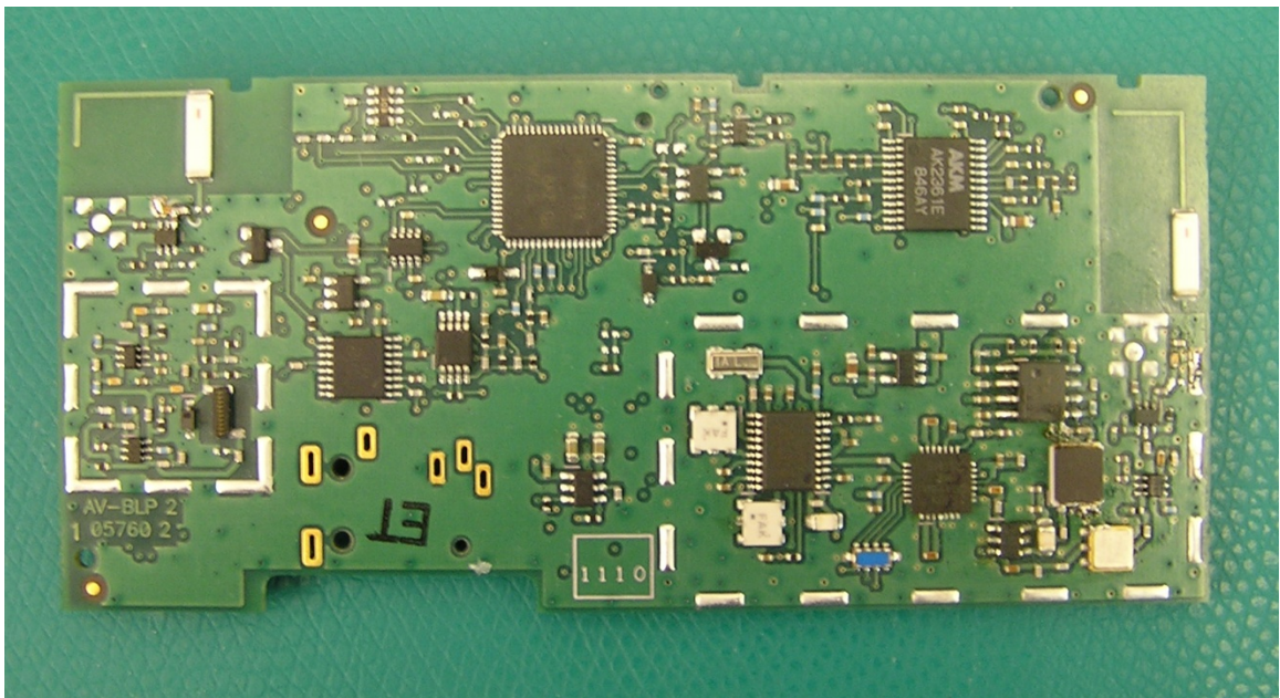
PCB FRONT without SHIELD
