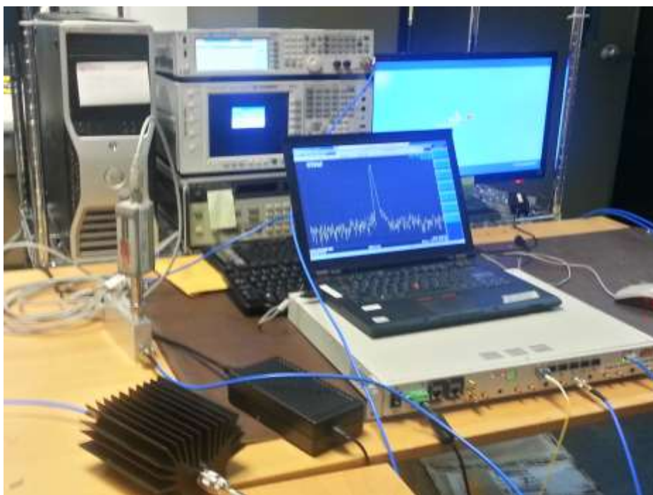
Figure 3 Conducted Test Setup – Measurement Instruments
