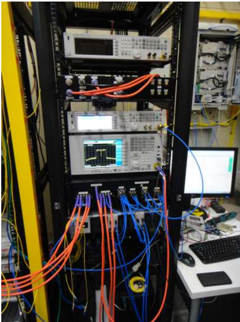
Figure 6: Conducted Test Setup – EUT
