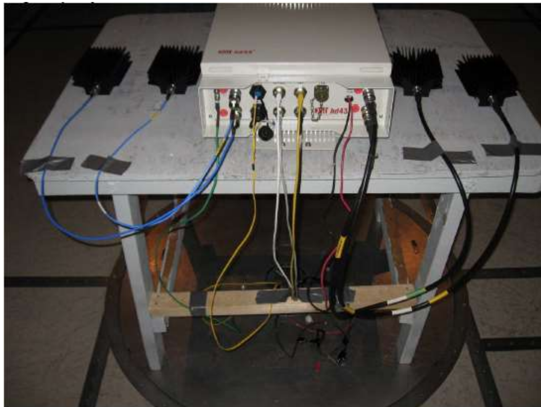
Figure 4: High Frequency measurements - Radiated Emissions Test Setup
