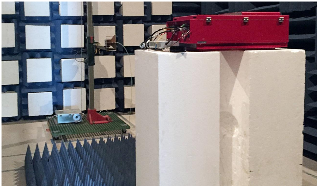
Figure 1: Radiated Emissions (Above 1GHz) Test Setup
