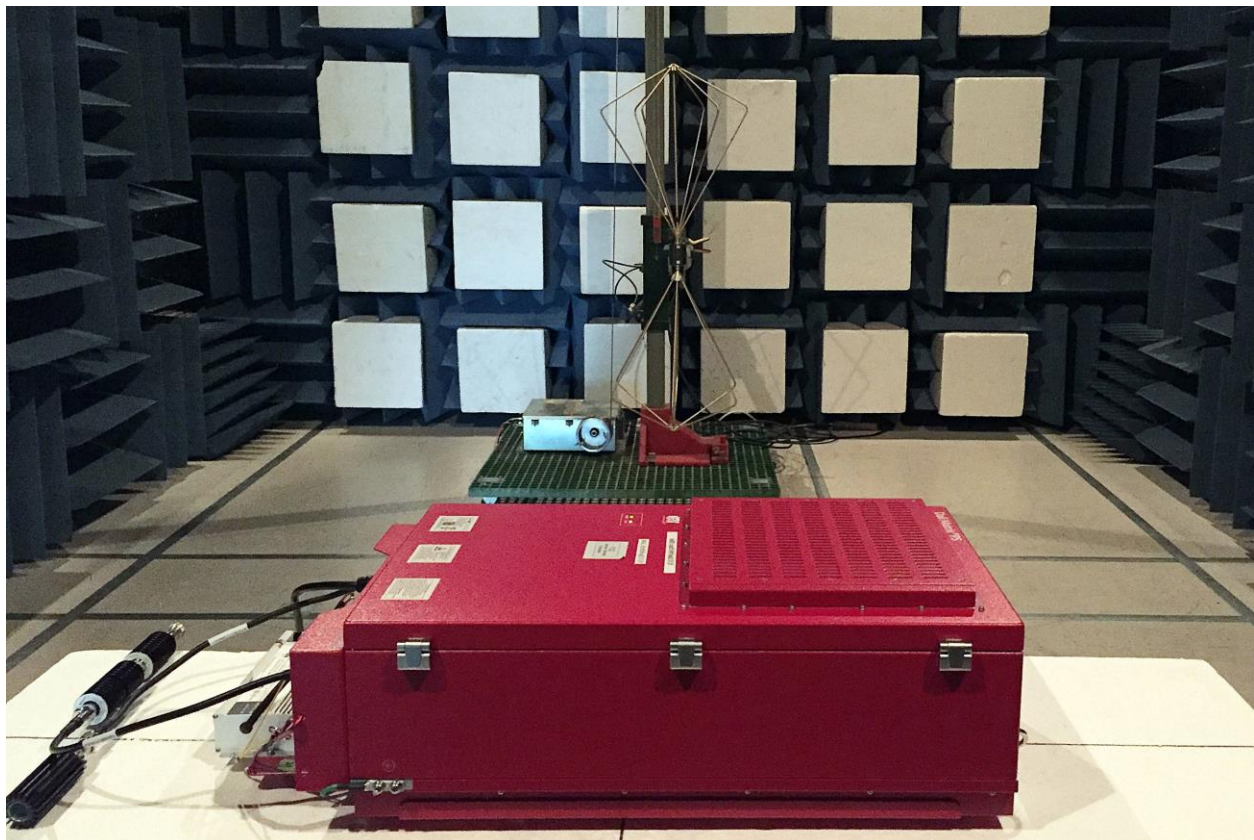
Figure 2: Radiated Emissions (30 to 250MHz) Test Setup
