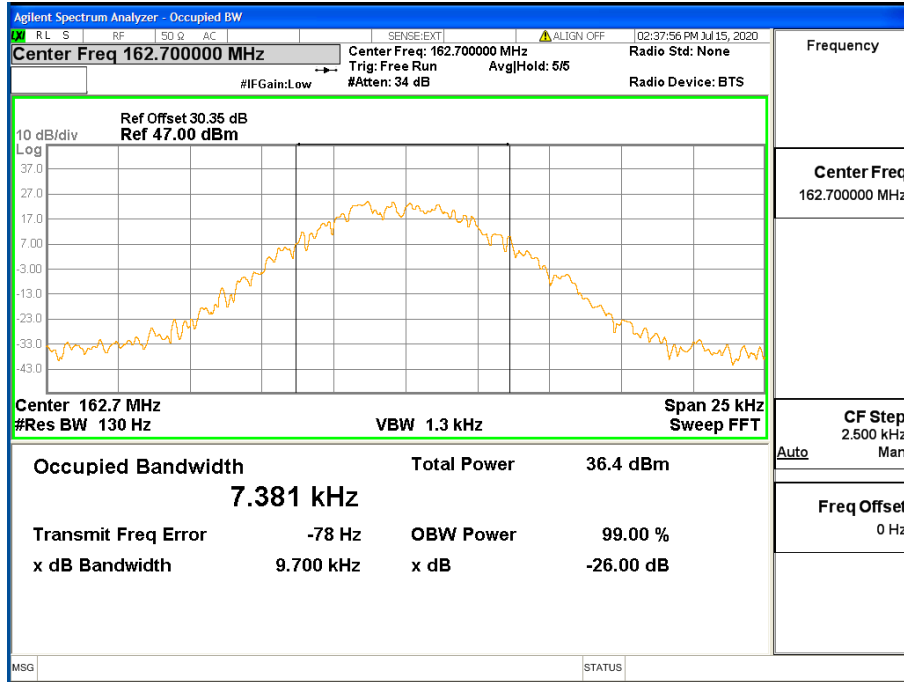
C4FM Signal at 162.7 MHz
