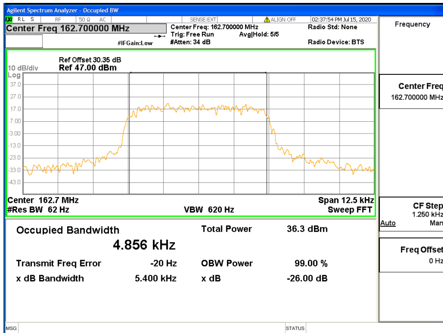
CQPSK Signal at 162.7 MHz
