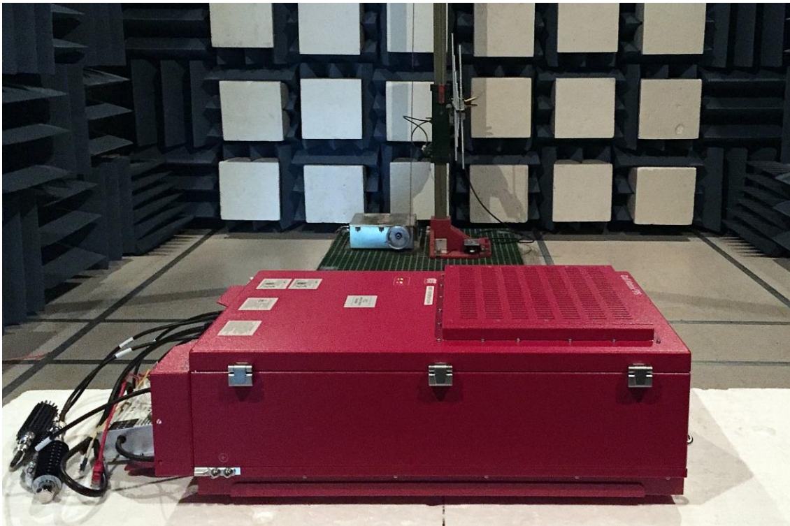
Figure 4: Radiated Emissions (Above 1GHz) Test Setup
