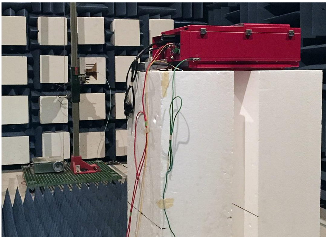
Figure 4: Radiated Emissions (Above 1GHz) Test Setup
