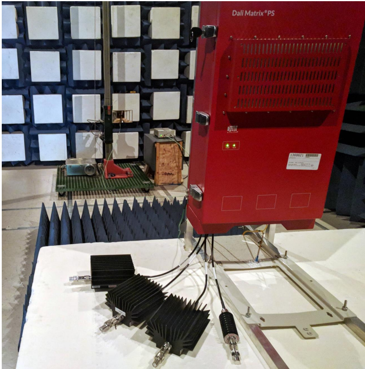
Figure 3: Radiated Emissions (Above 1GHz) Test Setup: Emissions on Cabinet
