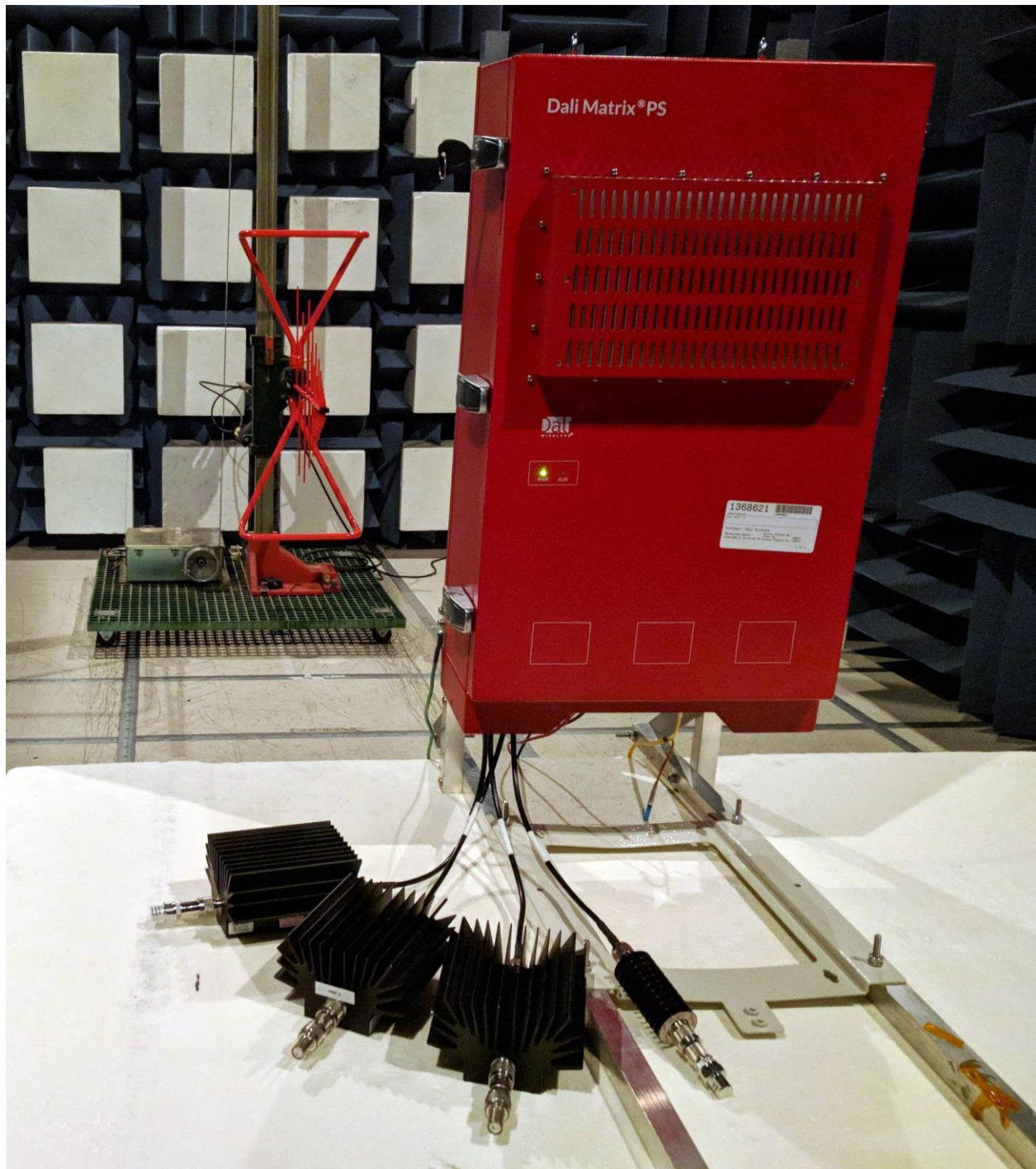
Figure 2: Radiated Emissions (Below 1GHz) Test Setup: Emissions on Cabinet
