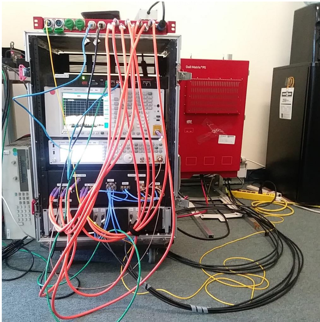
Figure 1: Conducted Test Setup – EUT
