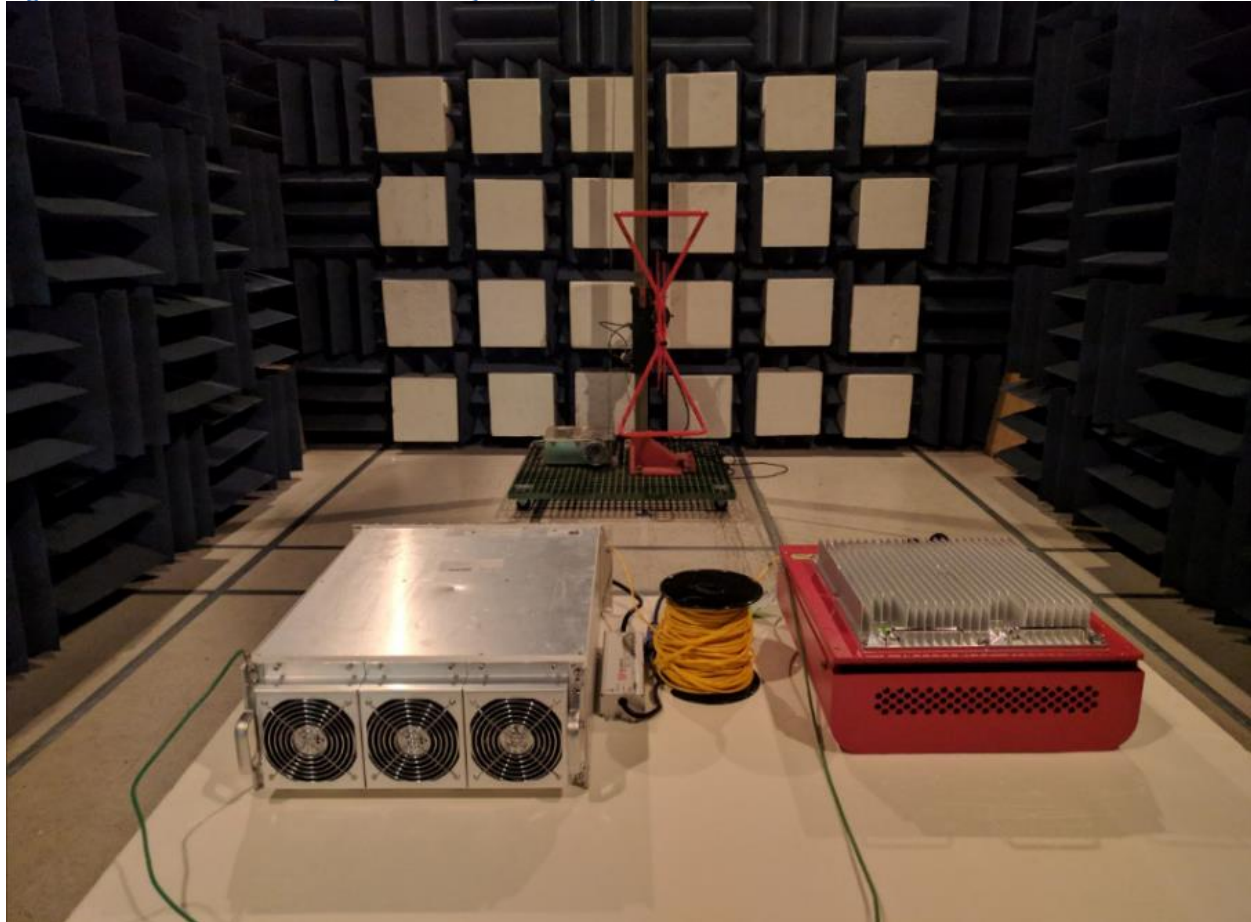
Figure 1: Radiated Emissions (Below 1GHz) Test Setup
