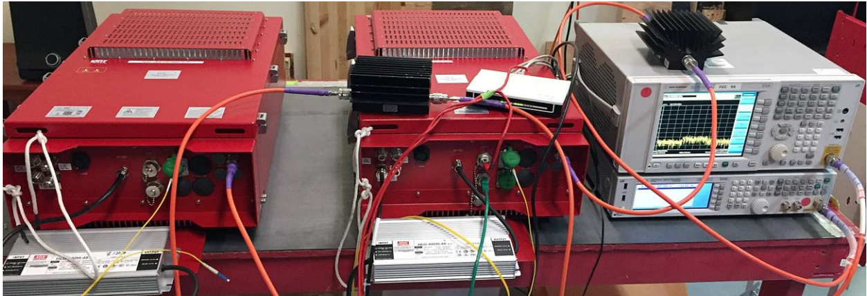
Figure 1: Conducted Test Setup – EUT
