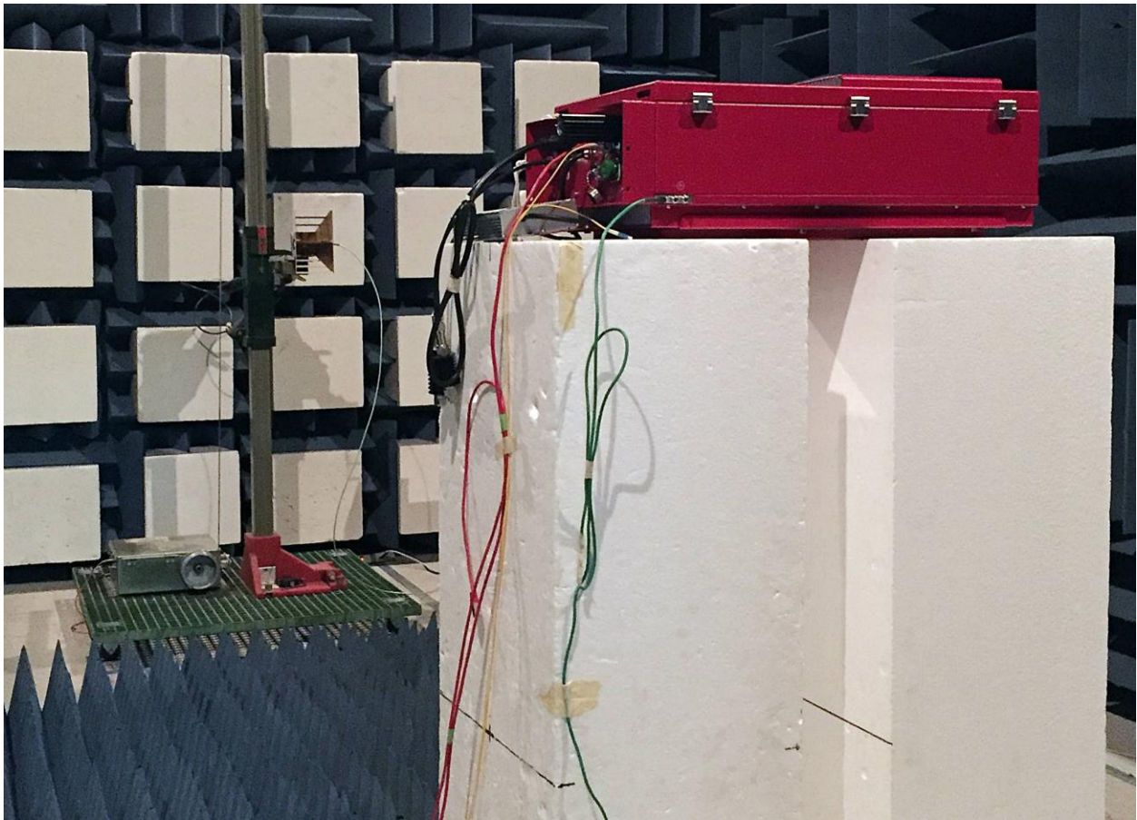
Figure 4: Radiated Emissions (Above 1GHz) Test Setup: Emissions on Cabinet
