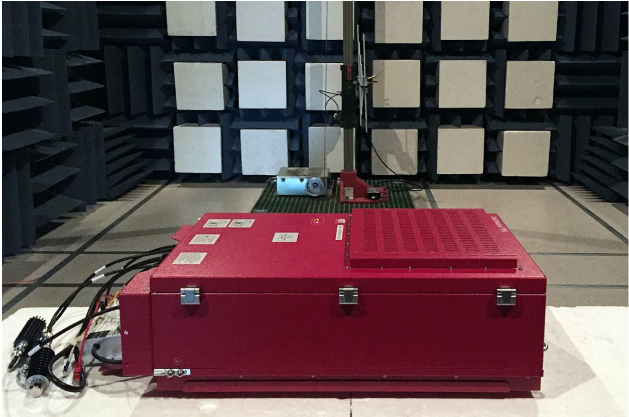
Figure 3: Radiated Emissions (300 to 1000MHz) Test Setup: Emissions on Cabinet
