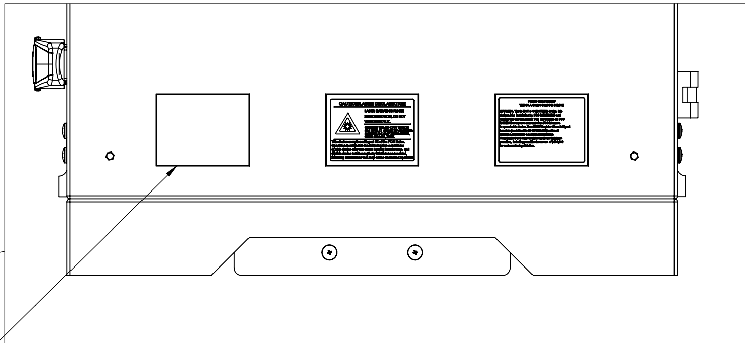
DETAIL A SCALE 2 : 5
