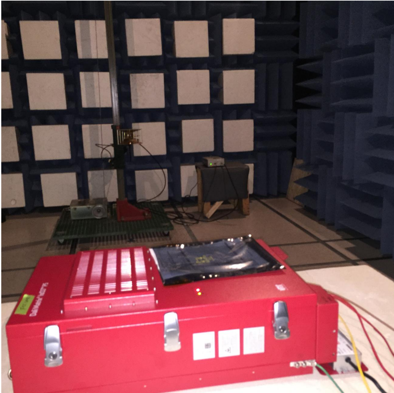
Figure 2: Radiated Emissions (Above 1GHz) Emissions Test Setup
