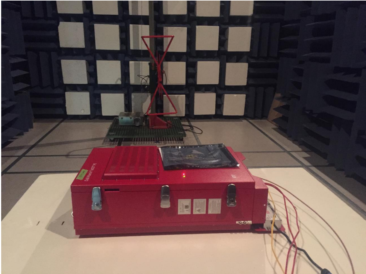
Figure 1: Radiated Emissions (Below 1GHz) Emissions Test Setup
