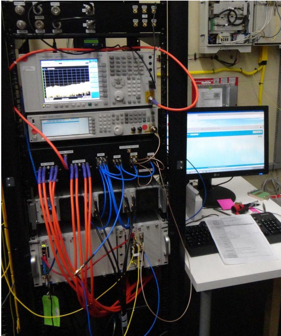
Figure 3: Conducted Test Setup – EUT
