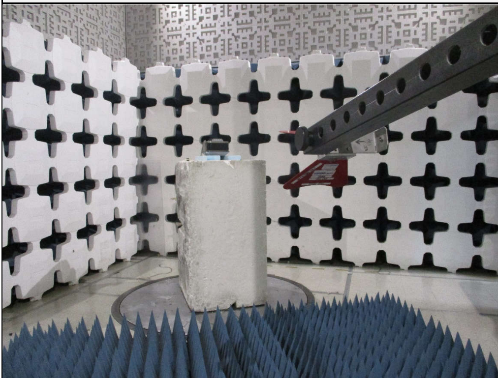
Test Setup for Spurious Radiated Emissions, 1GHz to 10GHz – Antenna Polarization Vertical
