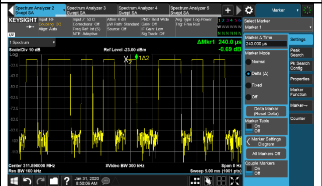
Duty Cycle 4#
