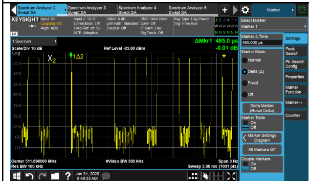
Duty Cycle 3#
