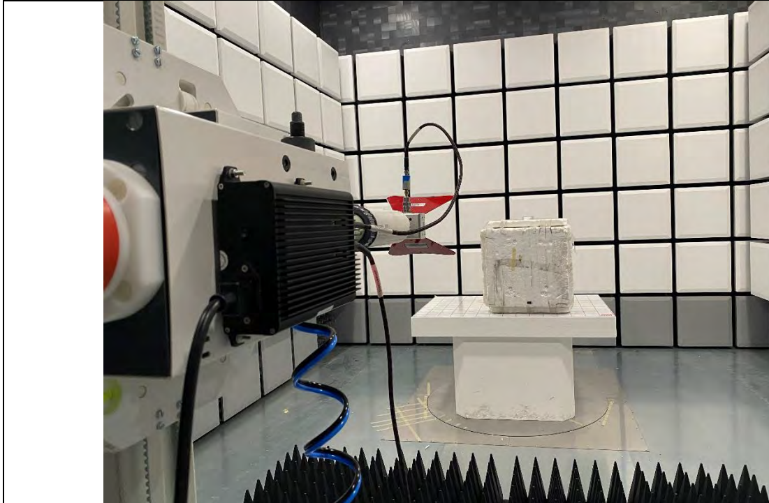
Radiated Emission Test above 1GHz Front View
