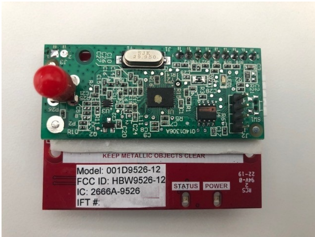
Assembly – Top
