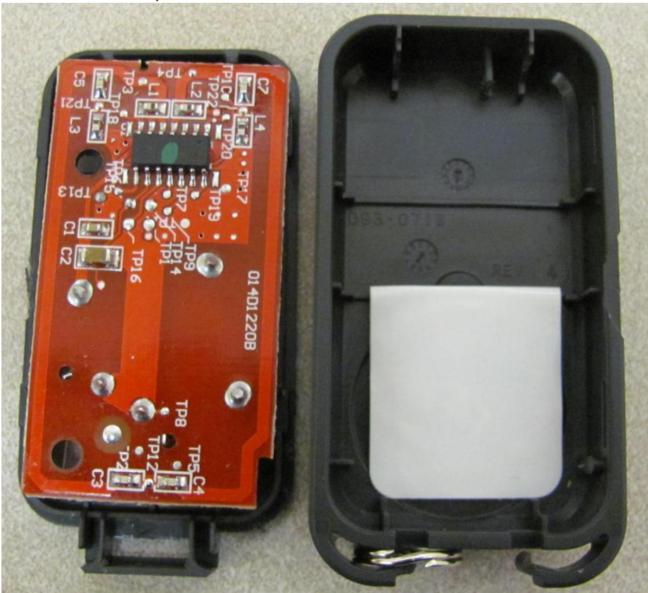
Internal showing the RFID passive coil (the white stick on inside the enclosure)
